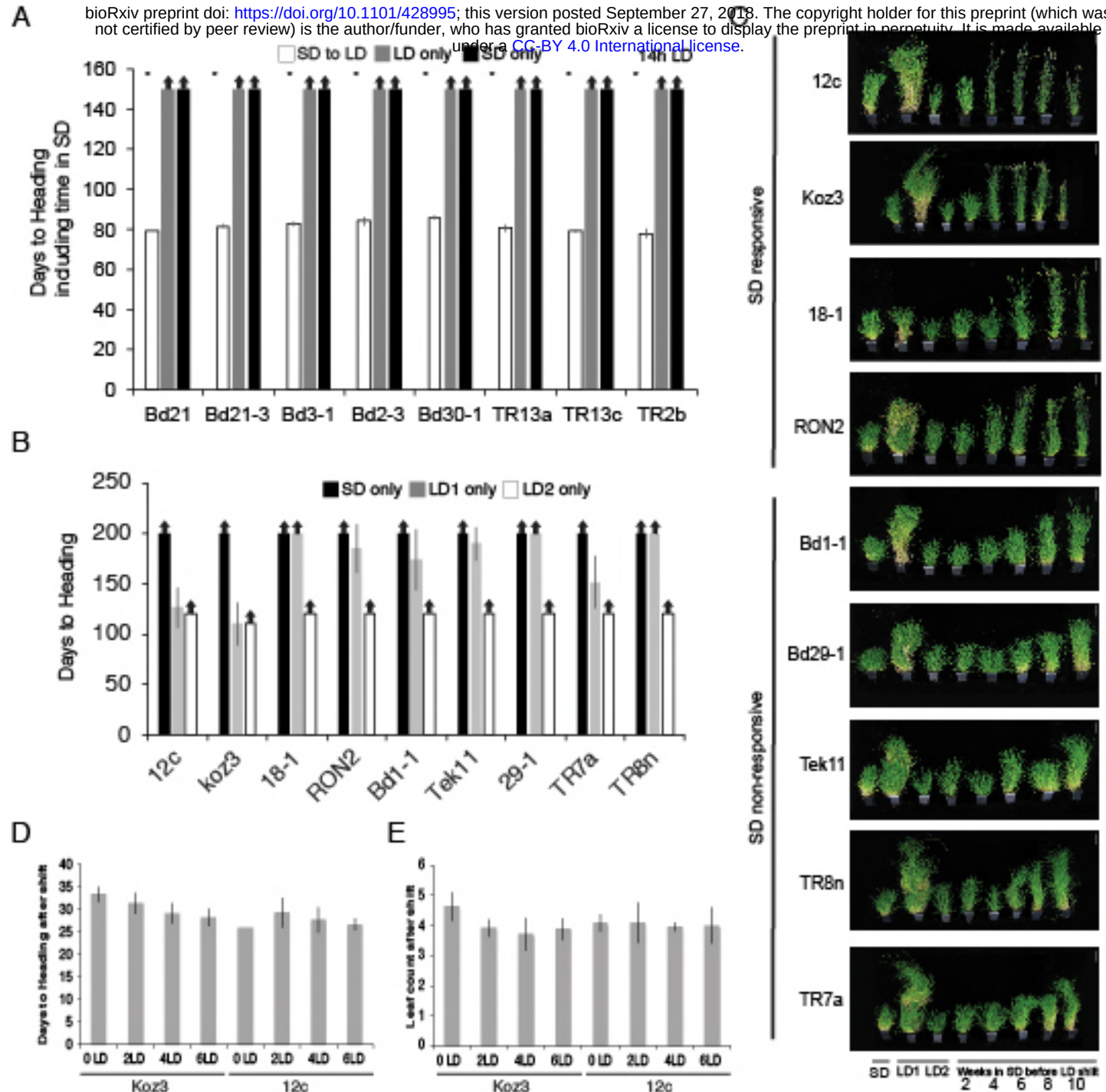
Figure 1-figure supplement 1. Natural variation in the short day vernalization response
