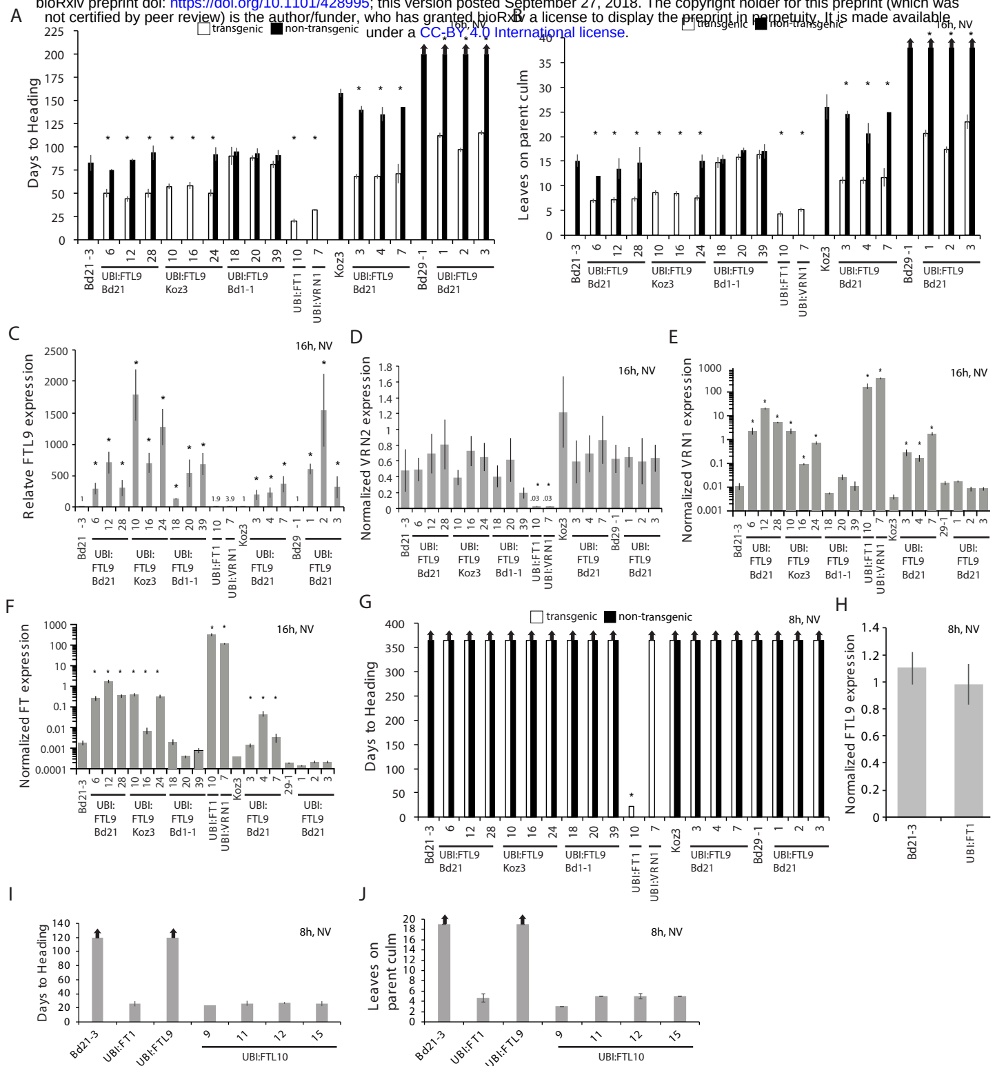
Figure 2-figure supplement 3. Effects of ubiquitin promoter-mediated constitutive expression of FTL9 , FTL10 , FT1 , and VRN1 (A-B) Flowering times as days to heading (A) or final leaf count on parent culm at time of flowering (B) of independent UBI:FTL9 transgenic lines (white bars) in Bd21-3 , Koz3 , and Bd29-1 compared with the respective wild-types and segregating non-transgenics (black bars). Lines with no non-transgenic plants are fixed for the transgene. Bars represent the average of at least 6 plants \pm SD. The experiment was repeated with similar results (data not shown). Arrows above bars indicate that none of the plants flowered at the end of the experiment. (C-F) Quantitative RT-PCR expression data from the upper leaf at the fifth leaf stage grown in a 16-h photoperiod. Expression data are normalized to UBC18 and represent the average of three biological replicates \pm SD. Expression analyses were repeated with similar results. Single asterisks indicate P-values < 0.01 . NV, non-vernalized. UBI:FT1 and UBI:VRN1 transgenics are described in (Ream et al., 2014). UBI:FTL9 Bd21 cDNA is from Bd21 , UBI:FTL9 Koz3 cDNA is from Koz3 and UBI:FTL9 Bd1-1 cDNA is from Bd1-1 . (G) Days to heading in 8h photoperiod non-vernalized (NV). Dissections on the parent culm revealed that the meristems were still vegetative after 150 days of growth in SD for all lines except UBI:FT1 which flowers rapidly. (H) Quantitative RT-PCR expression data from the upper leaf at the third leaf stage grown in a 8-h photoperiod in UBI:FT1 and Bd21-3 . (I) Flowering times as days to heading (J) or final leaf count on parent culm at time of flowering of 4 independent UBI:FTL10 T1 transgenic lines, UBI:FT1 (T2 generation) and UBI:FTL9 Koz3 line 10 from (A) in this figure (T1 generation).
