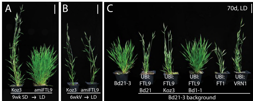
Figure 2. FTL9 is necessary for the SD vernalization response and sufficient to confer competence to flower. (A) amiFTL9 knockdown prevents SD vernalization. Koz3 wild-type and amiFTL9 knockdown plants grown in 8h SD for 9 weeks (9wk SD) before shifting into 20h LD. Bar= 5cm. (B) amiFTL9 knockdown has no effect on cold-mediated vernalization. Plants were vernalized as imbibed seed at 5°C for 6 weeks (6wkV) before outgrowth in 20h LD. Bar= 5cm. See Figure 2-figure supplement 1 for amiFTL9 details. All experiments were repeated with similar results. (C) Constitutive expression of dominant FTL9 alleles permits flowering in LD. Representative photo of Bd21-3 wild-type, UBI:FTL9 Bd21 (FTL9 from Bd21), UBI:FTL9 Koz3 (FTL9 from Koz3), UBI:FTL9 Bd1-1 (FTL9 from Bd1-1), UBI:FT1, and UBI:VRN1 grown in a 16-h photoperiod (LD) without cold or short day vernalization. All over expression lines are in the Bd21-3 background. Bar=5cm. See Figure 2-figure supplement 3 for UBI:FTL9 details including days to heading, leaf count data as well as mRNA expression analyses.
