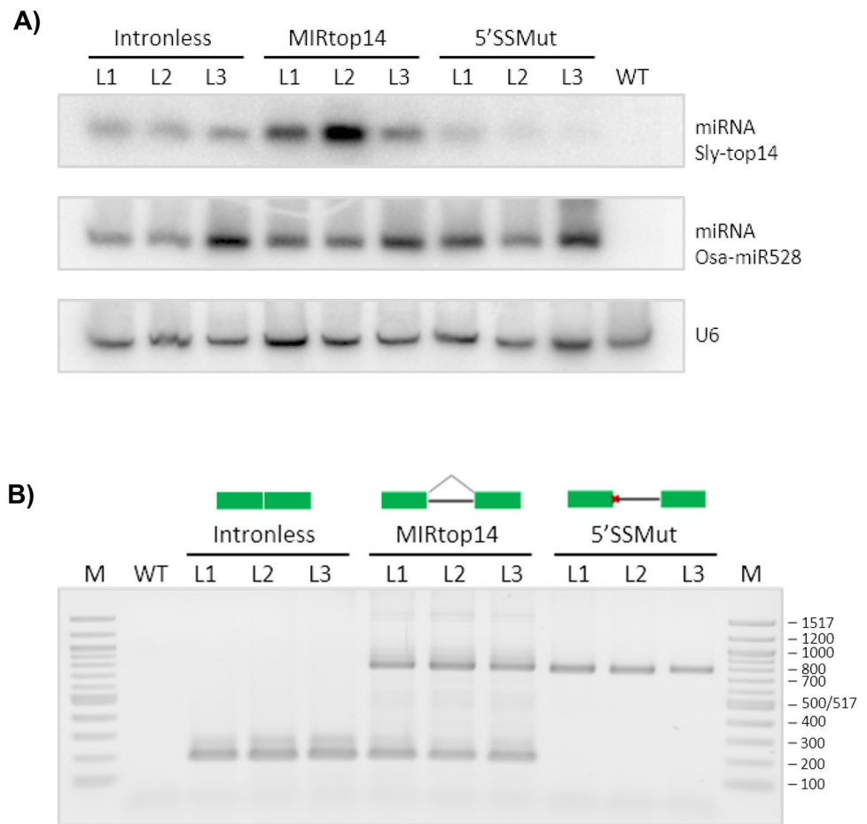
Fig. 5 Effect of the intron in mature miRNA Atop14 accumulation. A Northern-blot detection of mature miRNA Atop14 in A. thaliana wild type (WT) and A. thaliana transformed with the three MIRtop14 constructs (Intronless, MIRtop14 and 5'SSMUT). Three independent transgenic lines (L1, L2 and L3) were analysed per construct. Osa-miRNA528, that was part of the T-DNA, detection was included as internal control of gene expression. U6 detection was included as loading control. B Detection of pri-miRNA Atop14 in each sample after total RNA reverse transcription. Bands of 752 nucleotides correspond to the amplification of pri-miRNA Atop14 with intron and bands of 184 nucleotides correspond to the amplification of pri-miRNA Atop14 without intron. M, 100 bp marker; the size of the bands is given in base pairs (bp)
