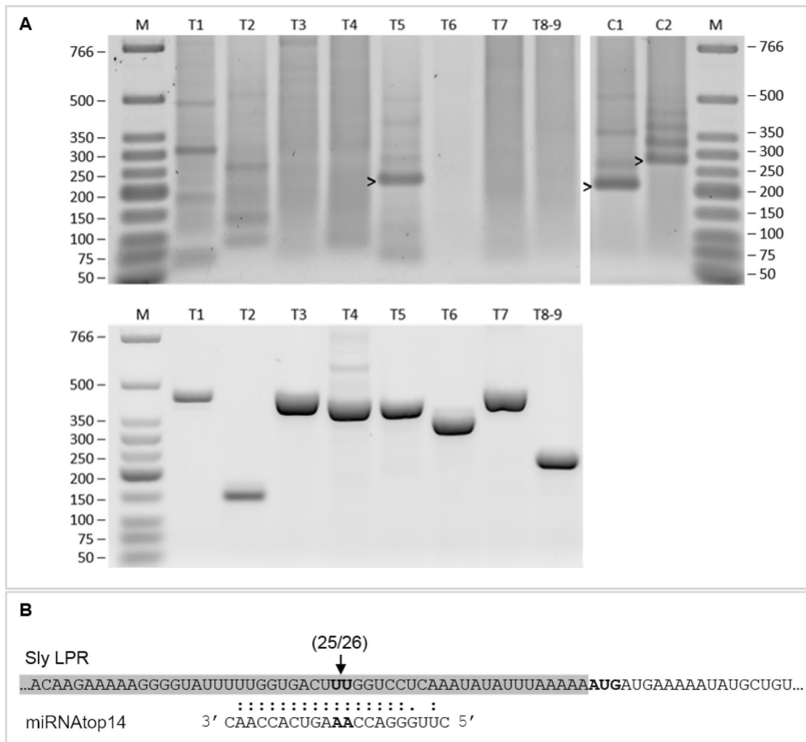
Fig. 6 RLM-RACE analysis and miRNAAtop14- LPR targeting in Solanum lycopersicum . A RLM-RACE analysis of the nine predicted targets predicted in Solanum lycopersicum , compiled in Table 1, each labelled with a target number (e.g., T1) according to Table 1. Target T8 and target T9 share the same sequence in the region of the putative miRNAAtop14 cleavage, so they could not be independently analysed (they have the same primers), and therefore, their common product is labelled as T8–9. Top Nested PCR products from RLM-RACE run in an agarose gel. Two control targets are included: C1, LA cleaved by miRNA319 and C2, GRAS24 cleaved by miRNA171. Bands showing the expected length are marked by an arrowhead (T5, C1 and C2). Expected product length from each target in nucleotides: T1=77, T2=145, T3=114, T4=145, T5=197, T6=158, T7=203, T8–9=140, C1=209, and C2=274. T1 and T2 show bands that are proximate to the expected amplicon size, so these bands were recov-
