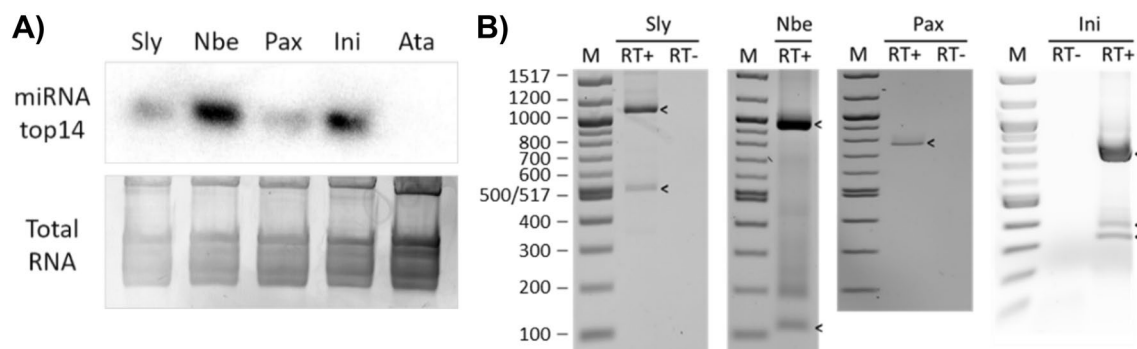
Fig. 4 Detection of miRNAAtop14 and pri-miRNAAtop14 in different plant species. A Detection of mature miRNAAtop14 in Arabidopsis thaliana (Ata) and four species of Solanales: Solanum lycopersicum (Sly), Nicotiana benthamiana (Nbe), Petunia axillaris (Pax), and Ipomoea nil (Ini) by northern blot. Ethidium bromide stained total RNA is included as loading control. B Detection of pri-miRNAAtop14 after total RNA reverse transcription in Sly and Pax, and mRNA reverse
