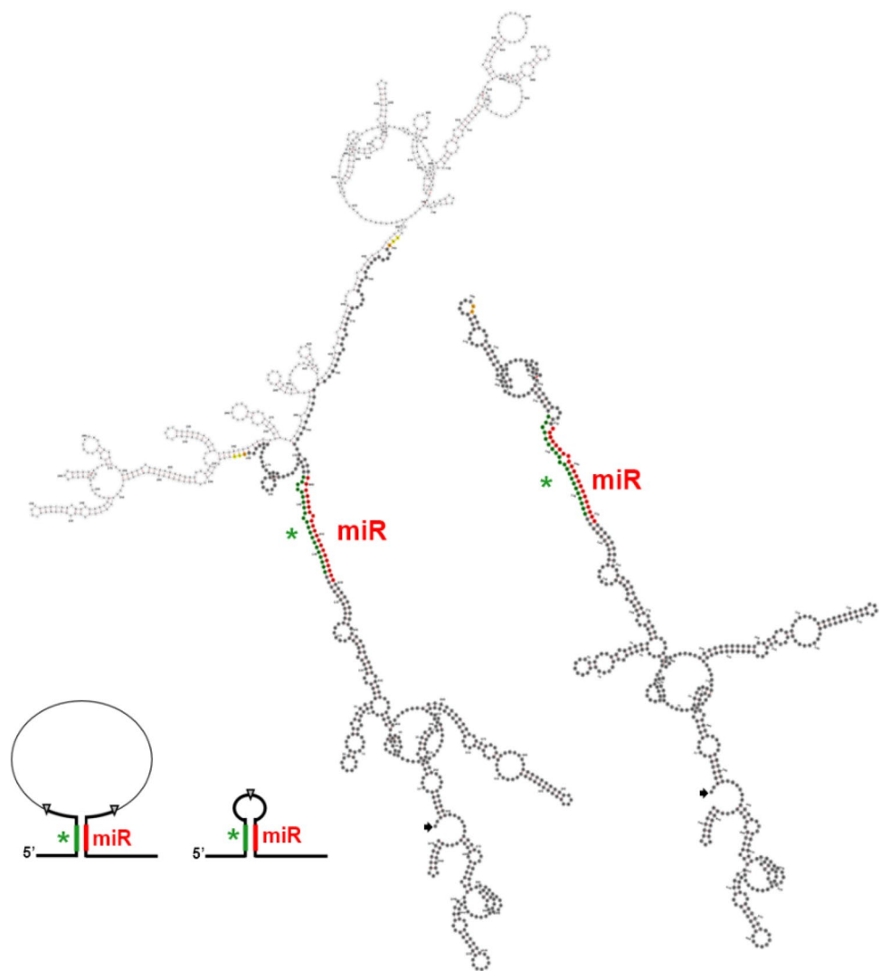
Fig. 2 pri-miRNA Atop14 secondary structure and schematic representation of the resulting miRNA hairpin, spliced (right), and non-spliced (left) variants ( Solanum lycopersicum ). pri-miRNA Atop14 secondary structure was predicted by RNAfold (Lorenz et al. 2011) as the one with minimum free energy from the putative pri-miRNA sequence and visualizations were created using forna tool (Kerpedjiev et al. 2015). miRNA Atop14 and miRNA Atop14* are indicated in red and green, respectively, in both the schemes and the secondary structure representation. In the schemes, exons are represented as bold lines, introns as thin lines, and SS and exon–exon junctions as grey triangles. In the secondary structure representations, nucleotides belonging to an exon are dark grey, while the ones within the intron are light grey. GU-AC dinucleotides at the SS are coloured yellow. First exon 3' end nucleotide and last exon 5' end nucleotide are coloured orange to mark the exon–exon junction after splicing. The first 5' residue of each transcript is indicated with a black arrow and the structures are always oriented with the miRNA stem-loop at the top
