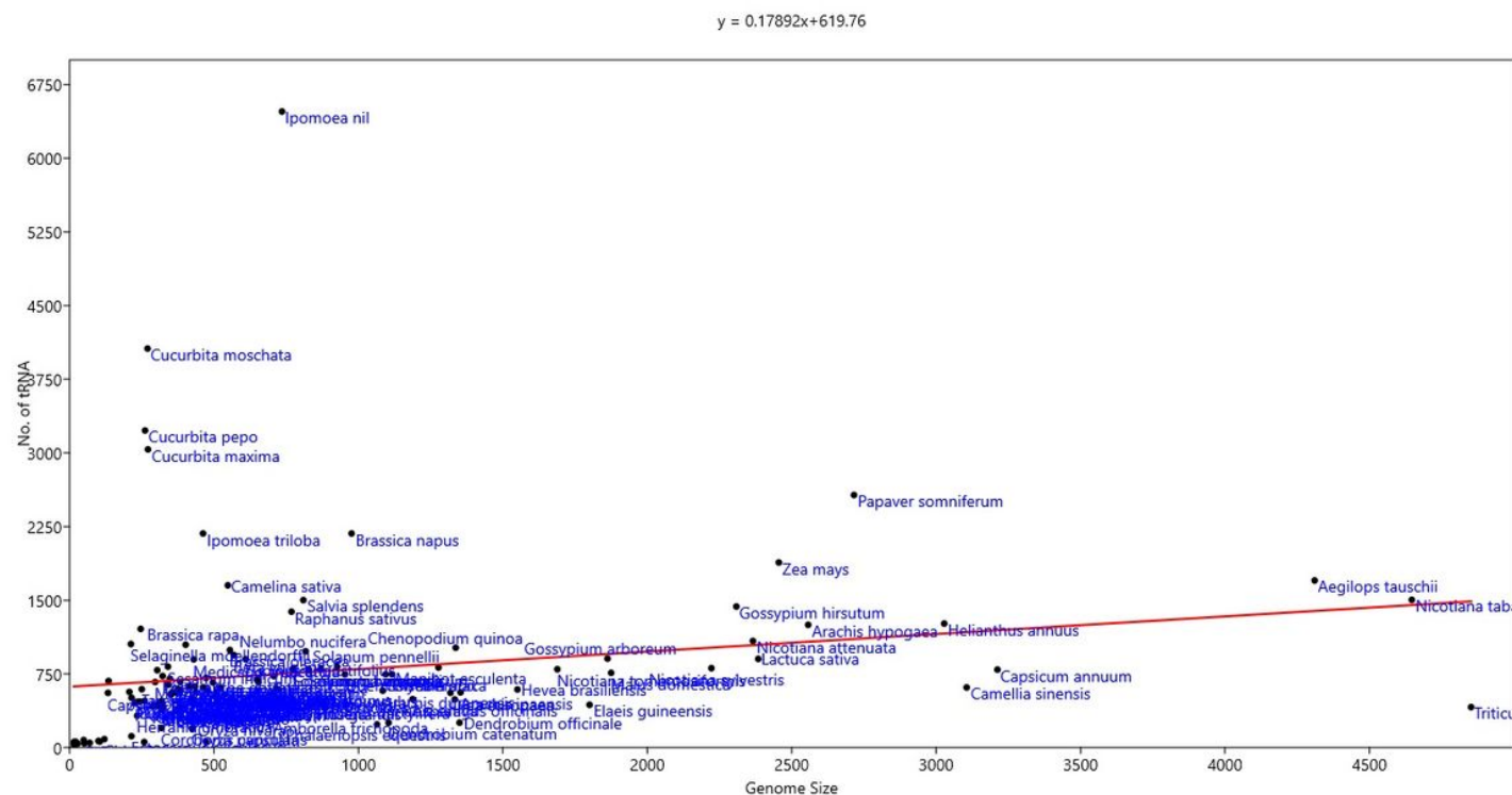
Figure 1 Regression analysis of tRNA gene number with plant genome. The analysis indicated that the number of tRNAs were not significantly correlated with plant genome size.
