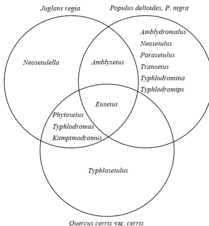
Figure 2. Genera of the mite family Phytoseiidae collected from walnut ( Juglans regia ), poplar ( Populus deltoides and/or P. nigra ) and oak ( Quercus cerris var. cerris in Samsun Province, Türkiye, between 2018 and 2022).
