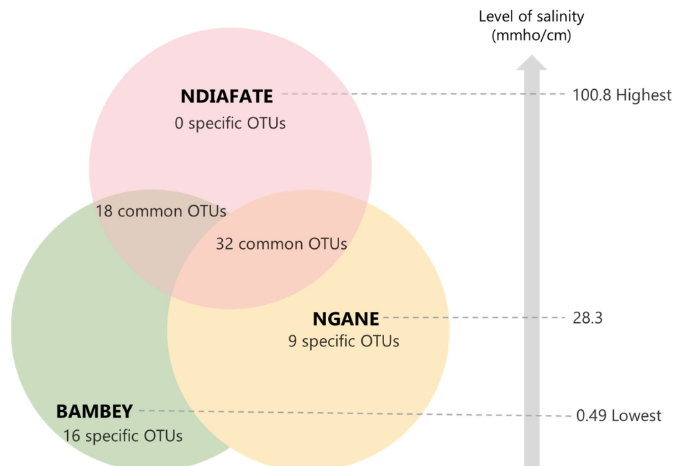
Figure 5. Venn diagram with specific or common OTUs recovered from Bambey, Ngane, and Ndiafate. Overlaps concern common OTUs.
