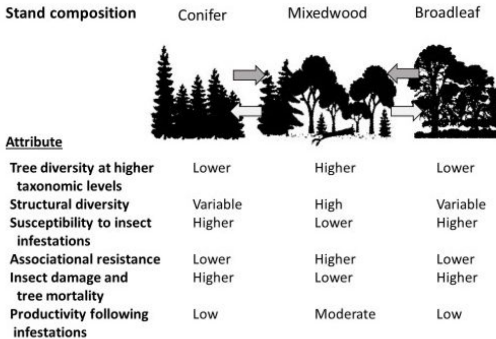
Fig. 1. Composition and attributes of conifer-dominated, mixedwood, and broadleaf-dominated stands. Mixedwood stands have greater diversity at higher taxonomic levels (e.g. family and above) that is more evenly distributed across co-dominant species, although not necessarily a greater number of species. Mixedwood stands typically have greater structural diversity than conifer- or broadleaf-dominated stands. Greater diversity at higher taxonomic levels confers reduced susceptibility to insect infestations, primarily through greater associational resistance. Depending on the insect, damage and tree mortality are reduced compared to conifer- or broadleaf-dominated stands. Successional changes in species composition favors either conifer or broadleaf dominance in the absence of major disturbances, depending upon forest type (indicated by the light arrows). In contrast, insect infestations and differential tree mortality can result in the formation of mixed composition stands (indicated by the darker arrows).
