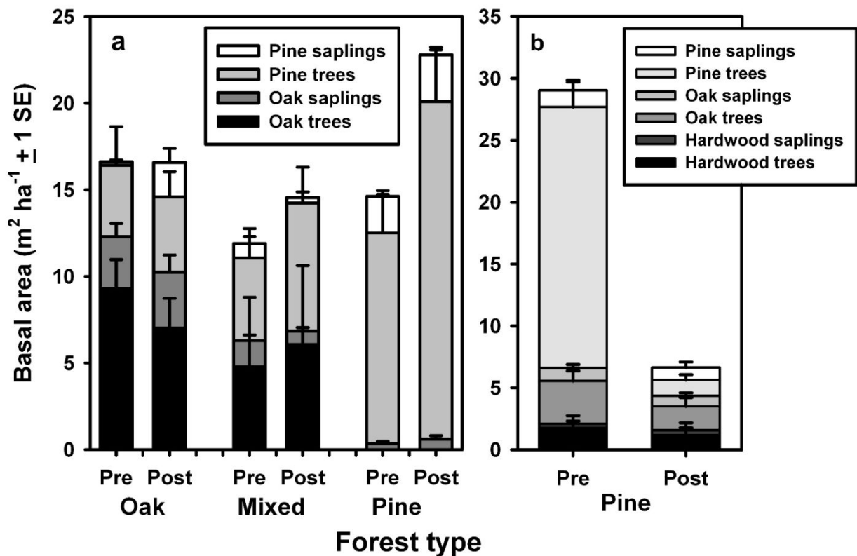
Fig. 3. a) Basal area of oak and pine trees and saplings pre-infestation (2004; 'pre') and a decade following infestations by gypsy moth (2018; 'post') in oak-dominated, oak-pine mixedwood, and pine-dominated stands. Dominant canopy trees were similar in age. Pre-infestation census data are from Clark et al. 2010, 2018, post-infestation from same sets of plots, unpublished data. b) Basal area of pine, oak and other hardwood trees and saplings pre- and post-infestation of southern pine beetle in pine-dominated stands (From Clark et al. 2017, 2020).
