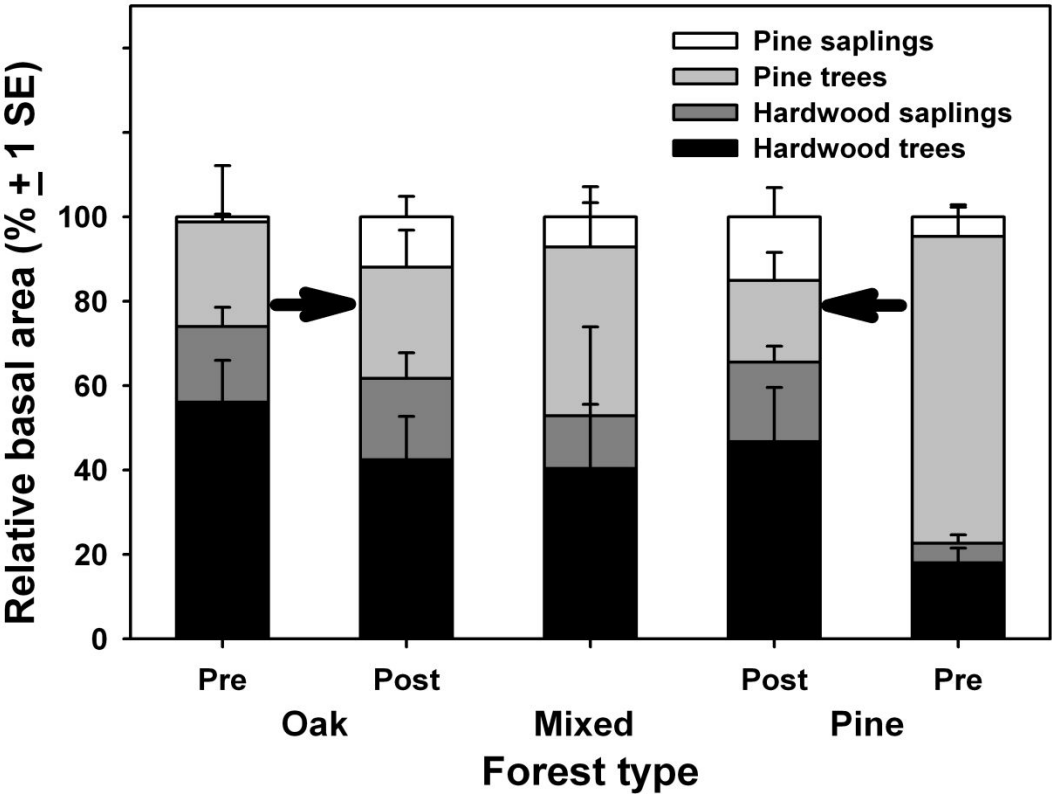
Fig. 4. Relative basal area of an oak-dominated stand before (pre-) and following (post) severe gypsy moth defoliation, an oak-pine mixedwood stand, and pitch pine stands before (pre-) and following (post) southern pine beetle infestation in the Pinelands National Reserve of New Jersey. Arrows indicate the directional changes in relative basal area caused by insect damage; the arrow on the left indicates gypsy moth damage and the arrow on the right indicates southern pine beetle damage. Adapted from census data in Clark et al. 2017, 2018, and 2020.
