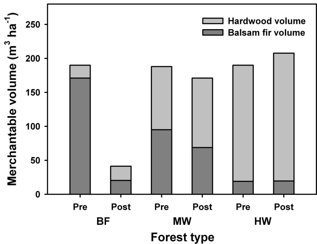
1032 Fig. 2. Merchantable volume of balsam fir and hardwood trees pre-infestation ('pre') and a 1033 decade following infestations by spruce budworm ('post') in balsam fir-dominated (BF), balsam 1034 fir-hardwood mixedwood (MW), and hardwood-dominated (HW) stands. Data were modified 1035 from Needham et al. (1999), where BF included 0-20% hardwood classes, MW included 30-70% 1036 hardwoods, and HW included 80-100% hardwoods.
