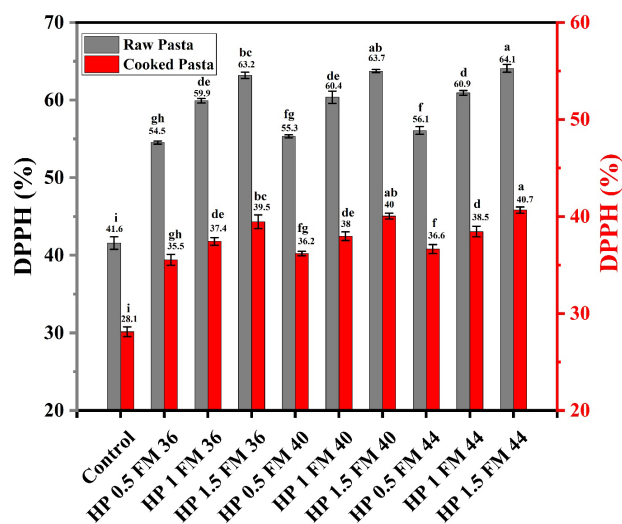
Figure 5. DPPH free radical scavenging results of raw pasta and cooked pasta. Different letter (a-i) in same color is significant different ( p < 0.05 ).
