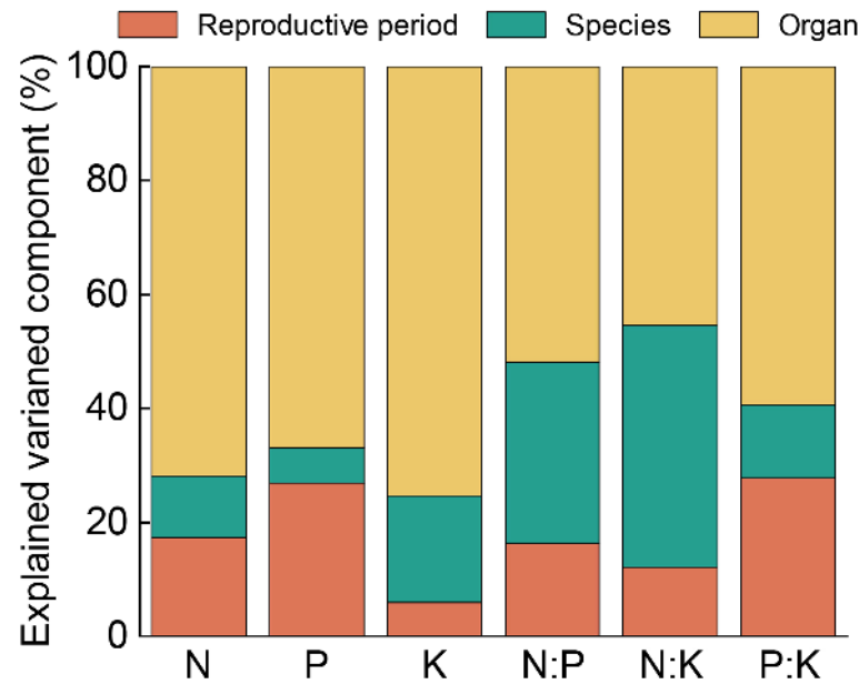
FIGURE 2 The hierarchical variance analysis of the six stoichiometric traits of the four Calligonum species.
