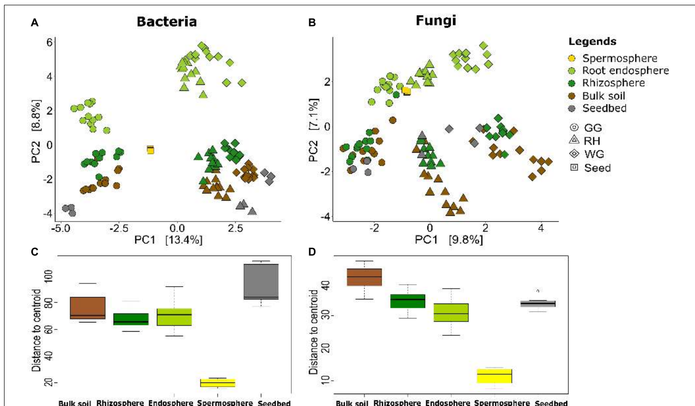
FIGURE 1 | Similarity and variation among microbial communities within compartments. Unconstrained ordination based on Euclidian distance matrices of bacterial (A) and fungal (B) communities across rhizosphere, root, bulk soil, and seedbed samples collected from wheat species ( A. tauschii , T. aestivum , T. dicoccoides , and T. durum ) in three locations (GG, Groß-Gerau; WG, Weilburger Grenze; RH, Rauischholzhausen) and seeds obtained from the gene bank labeled as Seed. Euclidian distance calculated from the data transformed to the centered log-ratio. The colors of the dots denote the compartments of the samples: rhizosphere (forest green), root (light green), bulk soil (brown), seed (yellow), and seedbed (gray). The box plots represent the range of distances from the centroid based on Euclidian distance matrices of bacterial (C) and fungal (D) compositions. The black lines in the box plots correspond to median values, and the dots indicate outliers.
