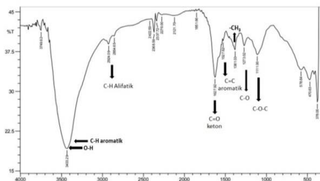
Figure 2. Infrared Spectrum (FT-IR) of Isolated Compounds
