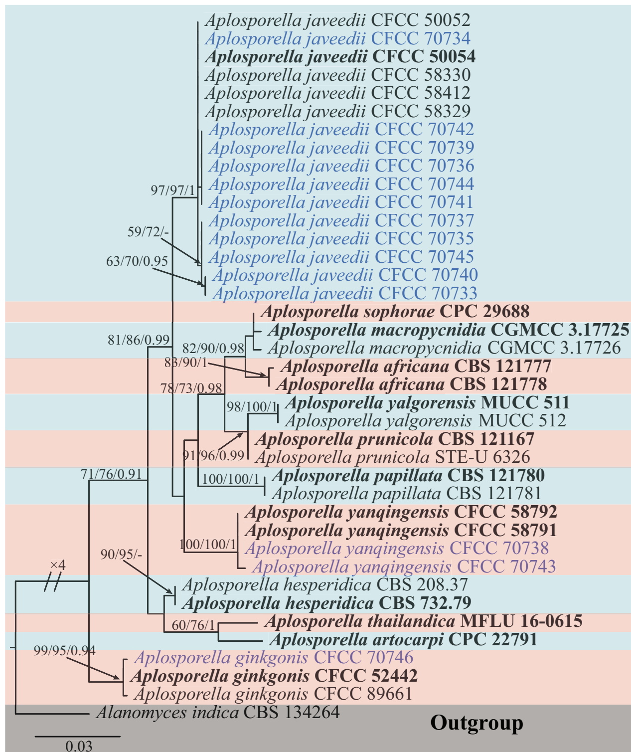
Figure 2. Phylogram generated from RAxML analysis based on ITS with tef1-α sequence data of Aplosporella isolates. The tree was rooted in Alanomyces indica (CBS 134264). The MP, ML ( \geq 50\% ), and BI ( \geq 0.9 ) bootstrap supports are given near the nodes, respectively. Isolates from this study are marked in blue, and ex-type strains are marked in bold.
