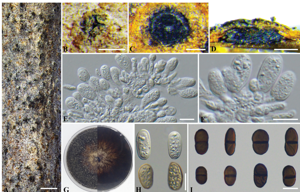
Figure 5. Dothiorella hortiarborum (BJFC-S1951) A, B habit of conidiomata on branch C transverse section of conidioma D longitudinal section through conidioma E, F conidiogenous cells and conidia G top (left) and bottom (right) sides of colonies on potato dextrose agar (PDA) H, I conidia. Scale bars: 1000 µm ( A ); 200 µm ( B–D ); 10 µm ( E–F, H–I ).
