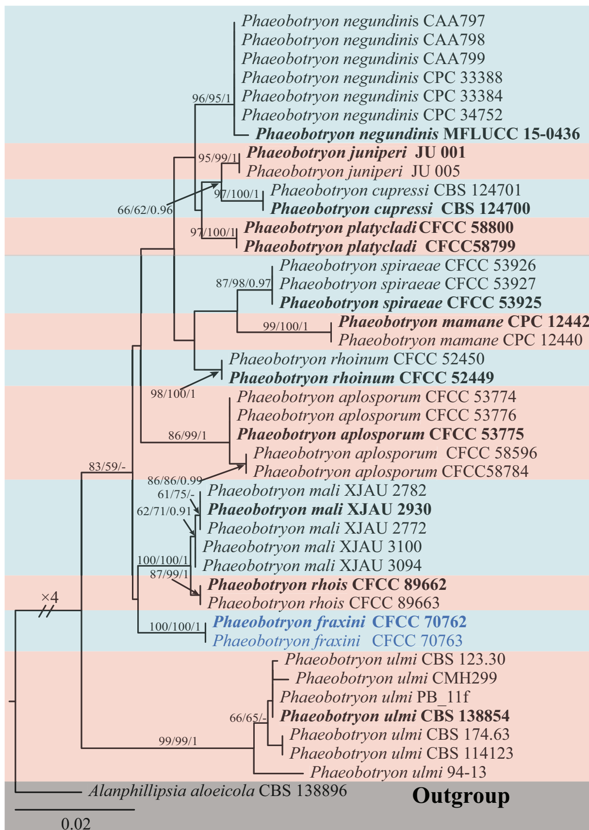
Figure 4. Phylogram generated from RAxML analysis based on ITS, LSU, and tef1-α sequence data of Phaeobotryon isolates. The tree was rooted in Alanphillipsia aloecicola (CBS 138896). The MP, ML ( \geq 50\% ), and BI ( \geq 0.9 ) bootstrap supports are given near the nodes, respectively. Isolates from this study are marked in blue, and ex-type strains are marked in bold.
