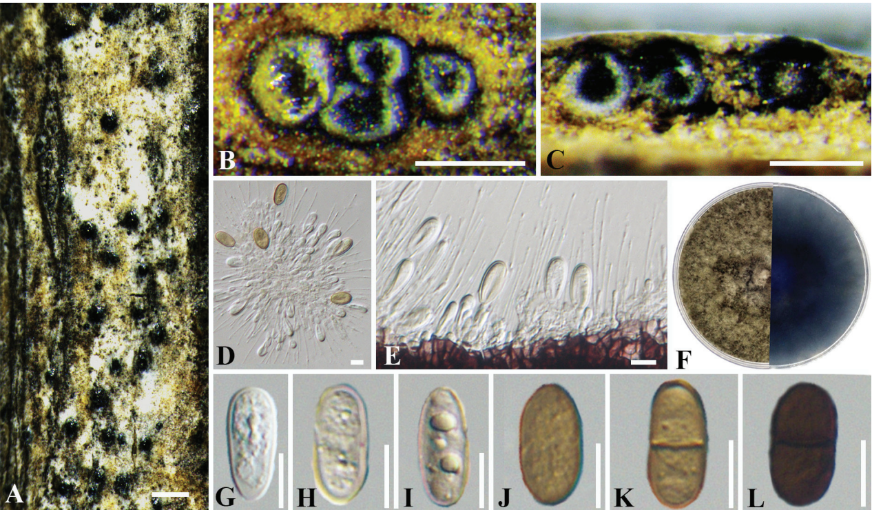
Figure 6. Phaeobotryon fraxini (BJFC-S1953) A habit of conidiomata on branch B transverse section of conidioma C longitudinal section through conidioma D, E conidiogenous cells and conidia F top (left) and bottom (right) sides of colonies on potato dextrose agar (PDA) G–L conidia. Scale bars: 500 \mu\text{m} ( A ); 200 \mu\text{m} ( B, C ); 10 \mu\text{m} ( D, E, G–L ).
