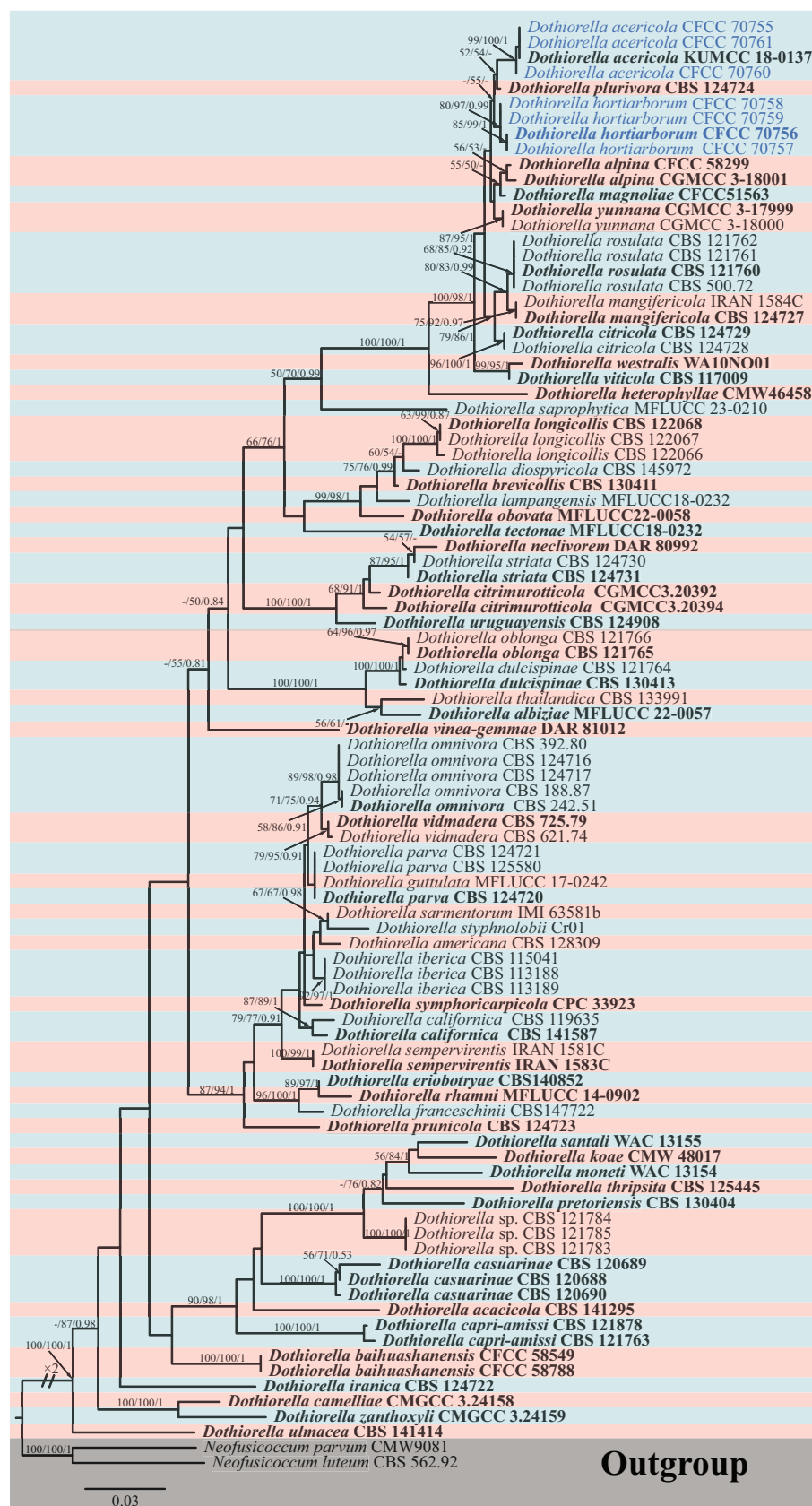
Figure 3. Phylogram generated from RAxML analysis based on ITS, tef1-a , and tub2 sequence data of Dothiorella isolates. The tree was rooted in Neofusicoccum luteum (CBS 562.92) and Neofusicoccum parvum (CMW9081). The MP, ML ( \geq 50\% ), and BI ( \geq 0.9 ) bootstrap supports are given near the nodes, respectively. Isolates from this study are marked in blue, and ex-type strains are marked in bold.
