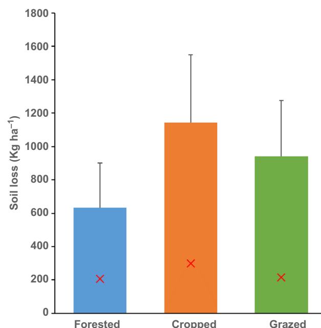
Fig. 2. Box and whisker plots showing observed soil loss ( \text{kg ha}^{-1} ) for seven common events for forested, cropped, and grazed catchments. Error bars represent s.d. ( \text{kg ha}^{-1} ), for forested (267), cropped (406), and grazed (336). \times represents mean of sediment yield data ( \text{kg ha}^{-1} , i.e. 208 (forested), 299 (cropped), and 215 (grazed)).
