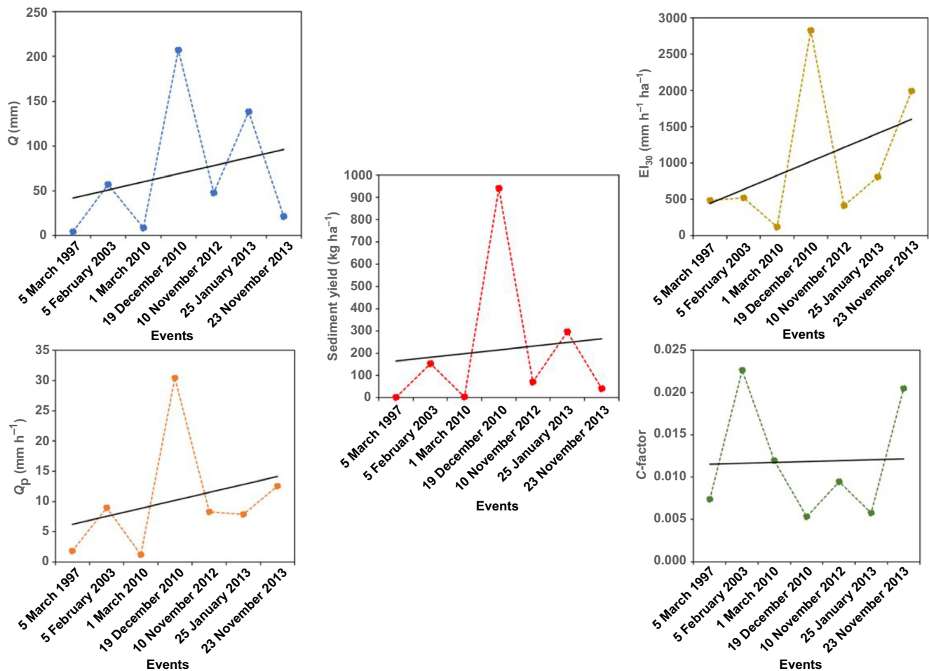
Fig. 3. Event-wise variation in event sediment yield with respect to the variation in El_{30} , Q , Q_p , and C for seven common events for grazed catchment.
