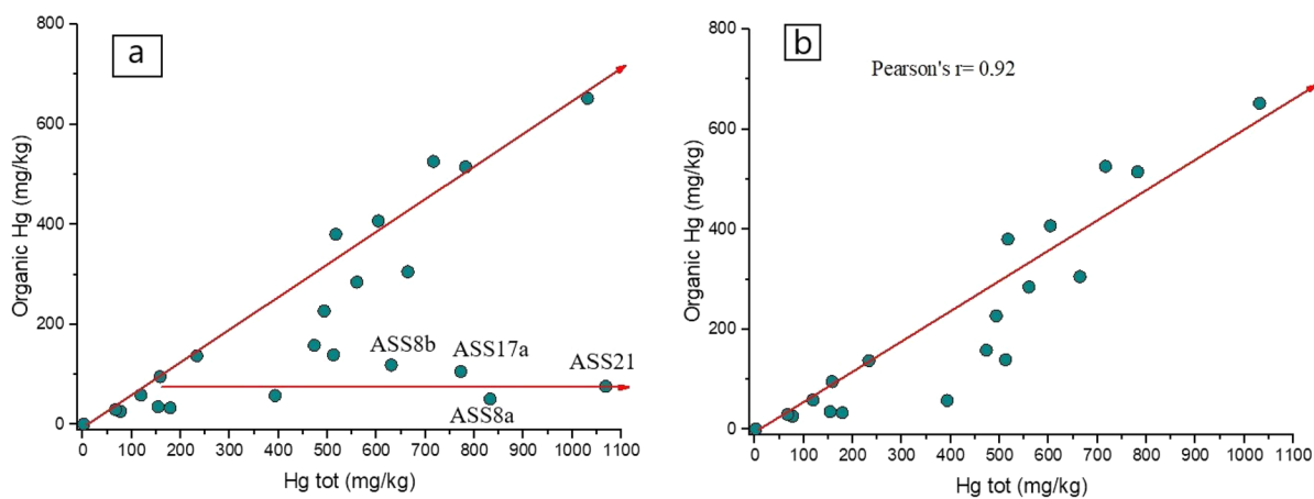
Fig. 3 Binary diagram between organic-related Hg vs. Total Hg (in \text{mg kg}^{-1} ) with a and without sampled ASS8a,b, ASS17a, ASS21 b . The organic Hg concentrations are those computed by thermal speciation
