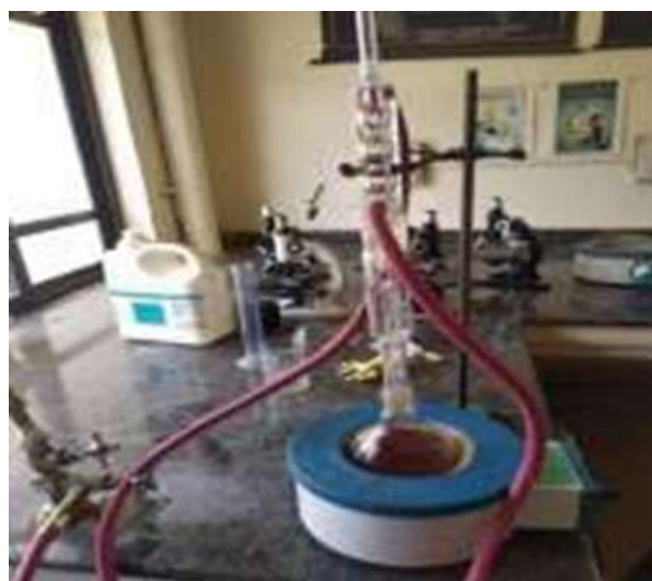
Fig No 2 Extraction of Colour Pigments
