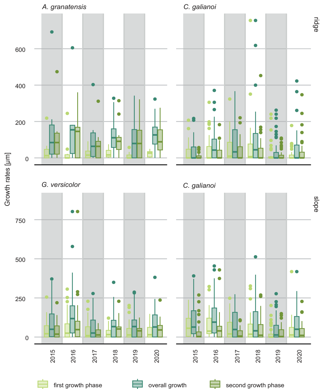
Fig. 15: Boxplot of growth phases showing the distribution of total annual growth (overall growth) as well as growth in the first and second growth phase in A. granatensis , C. galianoi and G. versicolor at different topographic positions. Alternating grey and white background markers highlight the years.
