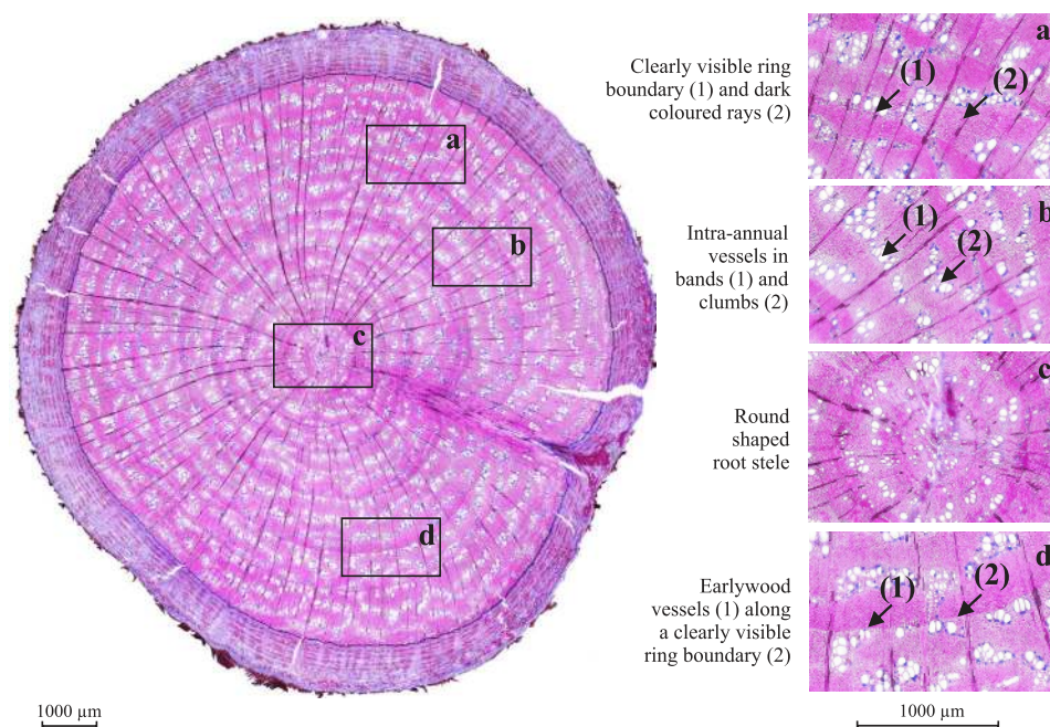
Fig. 5: Anatomical features in a root section of G. versicolor . The species' semi-ring porous xylem is characterized by a) clearly visible annual ring boundaries where thick-walled latewood cells merge into thin-walled earlywood cells. Narrow, dark coloured rays occur regularly and mostly range from the stele to the outer xylem boundary. b) Intra-annual vessels occur in clumps and bands and are surrounded by small parenchyma cells. c) The root stele is round shaped and d) the earlywood vessels are arranged along the ring boundaries.
