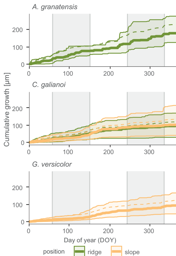
Fig. 14: Cumulative growth in C. galianoi , A. granatensis and G. versicolor at different topographic positions (ridges and slopes, see Fig. 12) shown as median (solid line), average (dashed line) and the 25% and 75% quartiles (shaded), over the days of the year using growth data of six consecutive years (2015 – 2020). Alternating grey and white background markers highlight the meteorological seasons.
