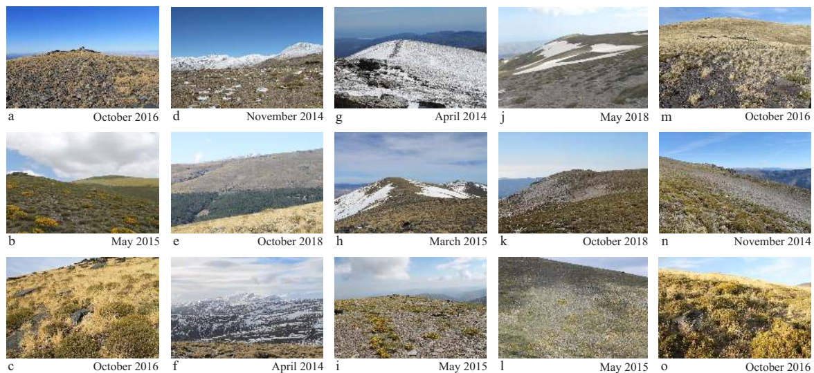
Fig. 8 Elevation and topography drive complex biogeographical patterns in our species. Vegetation cover and density increases along the elevation gradients from a) highest to b) intermediate and c) lowest elevations. During d) early winter and during f) spring, the highest peaks usually display a complex snow pattern with decreasing intensity towards e) the treeline. Ridges are generally characterized by the absence of snow cover, causing harsh conditions also during g) April and h) March, and therefore only show i) scarce vegetation cover. j) and l) Aspects of snowbeds during May, and k) during October indicate high inter-annual climate variability. Vegetation cover changes in dependence to topography from m) hilltops and n) snowbeds with low density to increasing density and thickness at o) slopes.
