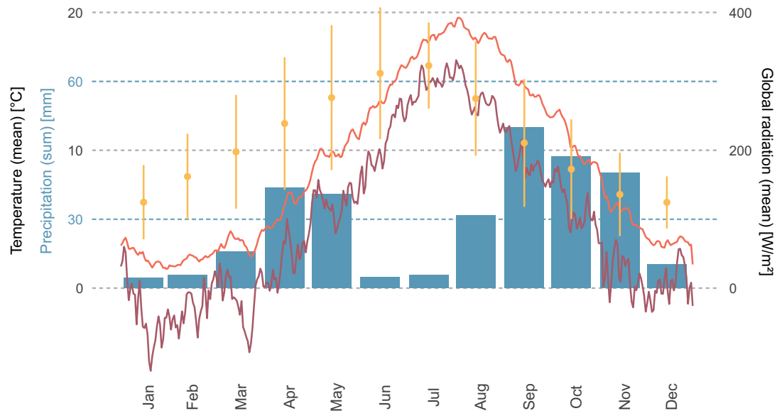
Fig. 9: Illustration of the overall climate regime. Monthly means of hourly measurements of global radiation (+/- SE, indicated by vertical lines), and precipitation (without snow), as well as daily means of air temperature (2 m above ground) measured at 2692 m a.s.l. and averaged over the period from 2015 to 2020, and soil temperatures measured at slopes across the entire elevation gradient and also averaged over the study period.
