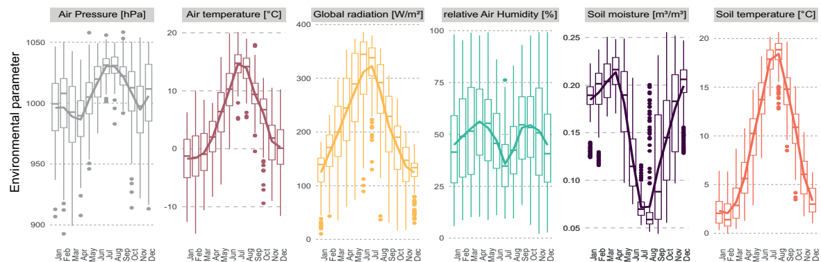
Fig. 10: Boxplots of hourly measurements of air pressure (AP), air temperature (T, 2 m above ground), global radiation (GRSZ, at 1 cm above ground in the shoot zone of one specimen), and relative humidity (rH) measured at 2692 m a.s.l. and averaged over the period from 2014 to 2020, and soil moisture and soil temperatures measured at slopes across the entire elevation gradient and also averaged over the study period.
