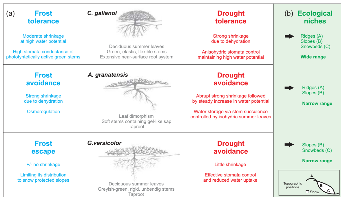
Fig. 17: (a) Growth strategies and mechanisms for coping with frost (blue) and drought (red) including drawings of the species C. galianoi , A. granatensis and G. versicolor and their most relevant traits (grey) determining the respective growth strategies and mechanisms. (b) Realised ecological niches of our focus species resulting from the respective growth strategies and mechanisms.
