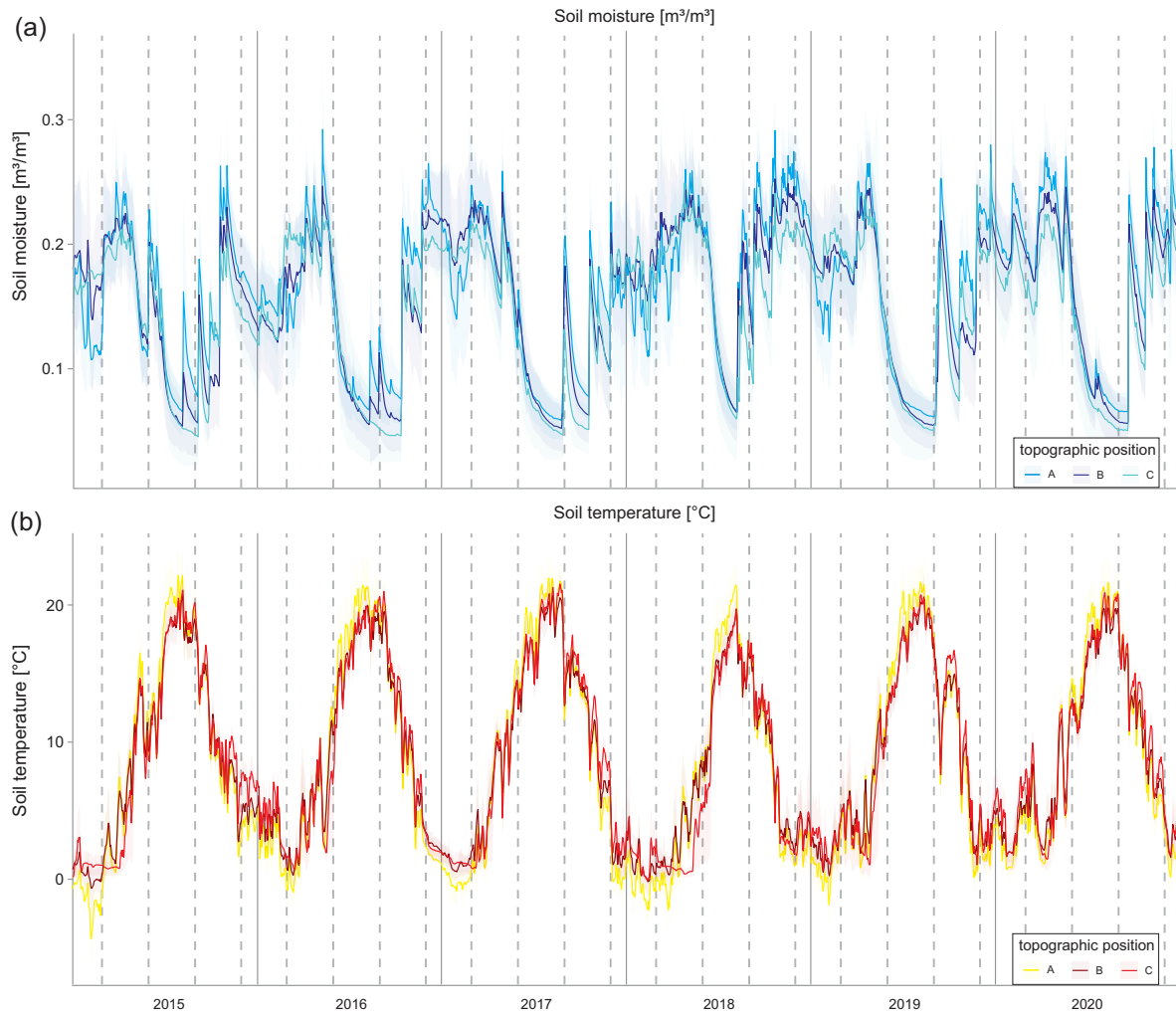
Fig. 11: Micro-environmental data, namely (a) soil moisture ( \text{SM}_{\text{RZ}} ) and (b) soil temperature ( \text{T}_{\text{RZ}} ), from three topographic positions (A = exposed ridges, B = slopes, and C = snowbeds). The presented curves represent averaged series and transparency indicates standard deviation. Vertical dashed grey lines indicate the seasons (namely: spring = March, April, May; summer = June, July, August; autumn = September, October, November; winter = December, January, February) and vertical black lines mark the years (modified after LÖFFLER et al. 2022).
