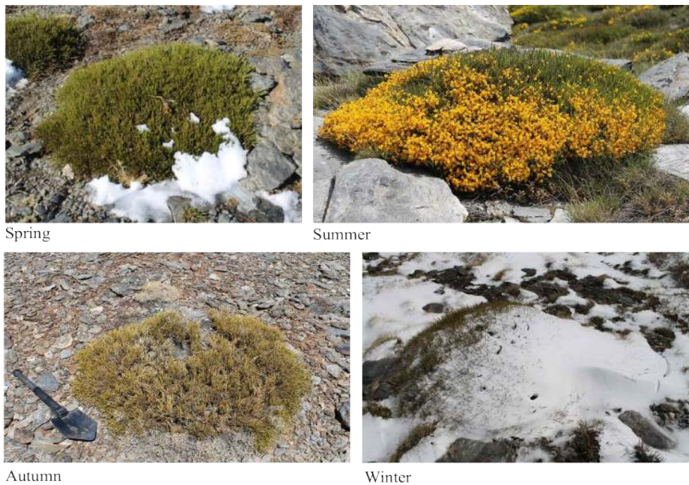
Fig. 2: Seasonal aspects of C. galianoi . In spring, when chlorophyll content is high, the species' stems appear intensely green, and in summer, its appearance is dominated by its yellow flowers. In autumn, it appears more brownish, and in winter, it is either covered by snow (slopes and snowbeds) or exposed to strong winds, low temperatures and occasional freezing conditions (ridges).
