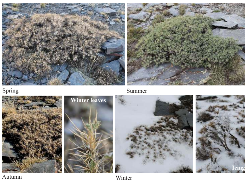
Fig. 6: Seasonal aspects of A. granatensis . In spring, the species is leafless, and at the beginning of summer, its appearance is dominated by its green summer leaves (first leaf cohort), which are shed towards the end of summer. At the beginning of autumn, it appears yellowish-brown, and towards the end of autumn, it becomes green again when winter leaves are unfolded (second leaf cohort). During winter, when the first frosts provoked leaf shedding, the species is either covered by snow (slopes), or exposed to strong winter winds, low temperatures and freezing, which in combination can lead to icing (ridges).
