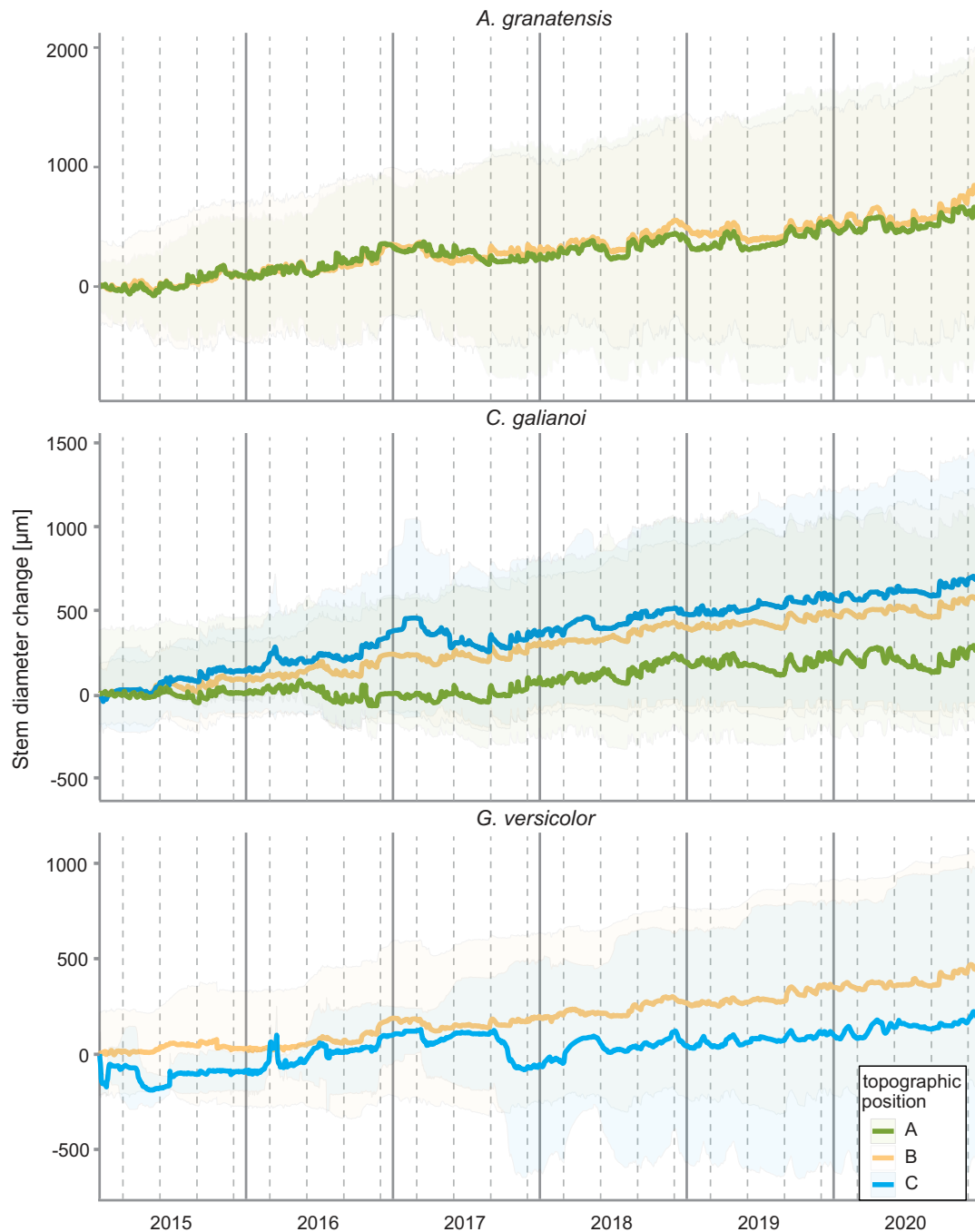
Fig. 12: Dendrometer curves representing averaged series of stem diameter change between A. granatensis , C. galianoi and G. versicolor as well as between ridges (A), slopes (B) and snowbeds (C); transparency indicates standard deviation among specimens. Vertical dashed lines indicate the meteorological seasons (namely: spring = March, April, May; summer = June, July, August; autumn = September, October, November; winter = December, January, February) and vertical solid lines mark the years (modified after LÖFFLER et al. 2022).
