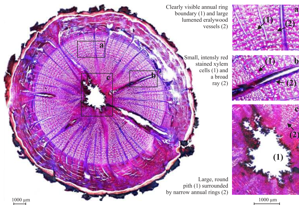
Fig. 7: Anatomical features in a stem section of A. granatensis . The ring porous to semi-ring porous xylem is characterized by a) clearly visible ring-boundaries marked by narrow band blue-stained marginal parenchyma bands and a row of large-lumened earlywood vessels. b) The xylem consists of small red-stained thick-walled cells with single vessels, and is crossed by wide rays containing a gel like cell sap. c) The comparatively large pith is round shaped and surrounded by cells containing dark staining substances.
