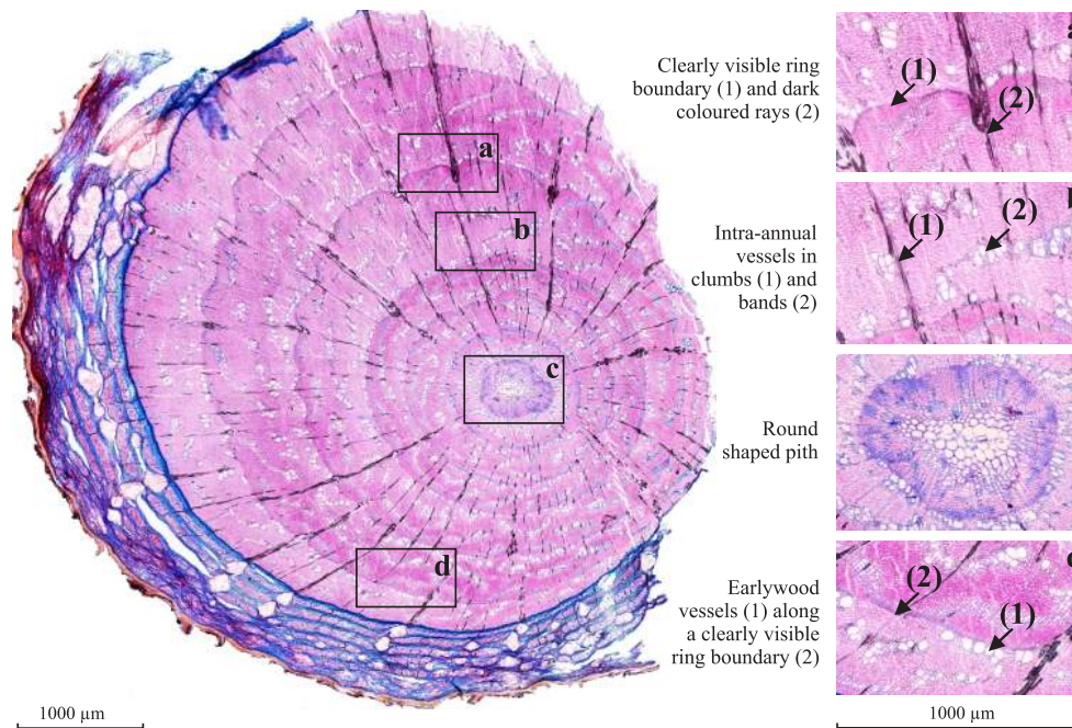
Fig. 3: Anatomical features in a base section of C. galianoi . The species' semi-ring porous xylem is characterized by a) clearly visible annual ring boundaries where thick-walled latewood cells merge into thin-walled earlywood cells. Narrow, dark coloured rays occur regularly and mostly range from the pith to the outer xylem boundary. b) Intra-annual vessels occur in clumps and irregular bands and are surrounded by small parenchyma cells. c) The pith is round shaped and d) the earlywood vessels are arranged along the ring boundaries.
