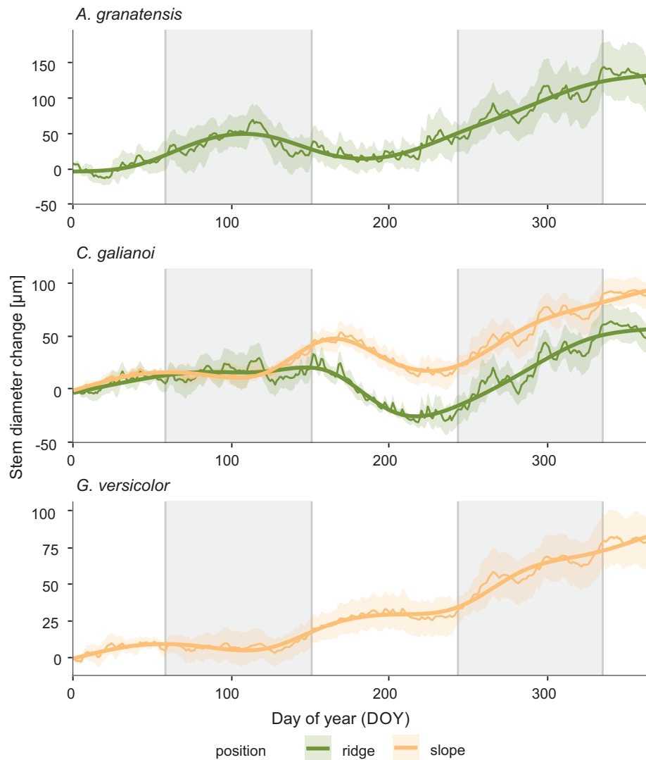
Fig. 13: Seasonal patterns of stem diameter change in A. granatensis , C. galianoi , and G. versicolor at different topographic positions (ridges and slopes, see Fig. 12) averaged over the studied period 2015 – 2020 and represented by generalized additive models (GAMs). Alternating grey and white background markers highlight the meteorological seasons.
