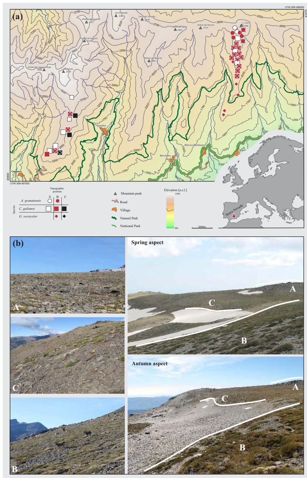
Fig. 1: (a) Topographic map of the Sierra Nevada showing the investigated mountain region and the locations of the sampling sites at ridges (A), slopes (B) and within snowbeds (C) along the elevational gradient (modified after Löffler et al. 2022). (b) Photos of the alpine environment showing the different topographic positions (modified after ALBRECHT et al. 2024a).
