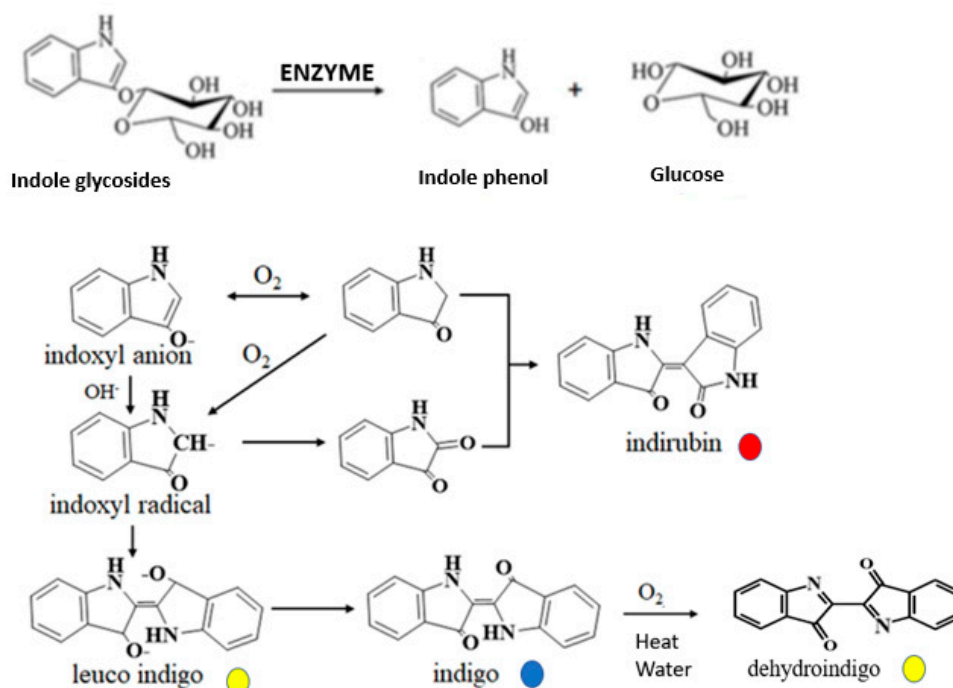
Figure 8. Possible pathways for various dye molecule production. The corresponding color of each component is indicated.
