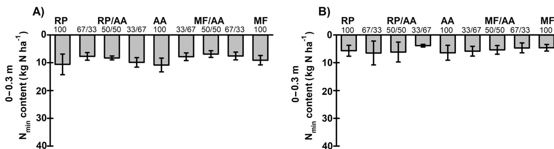
FIGURE 2 Plant-available mineral nitrogen ( N_{\min} ) content ( \text{kg N ha}^{-1} ) at a 0- to 0.3-m soil depth in field trials in 2019 and 2021: (A) on June 27, 2019, p = 0.06 ; and (B) on May 25, 2021, p = 0.66 . One-factor analysis with Tukey's honestly significant difference (HSD). Means \pm standard deviation. Numbers 67/33, 50/50, and 33/67 indicate mixture proportions in percent, and 100 indicates a pure stand. AA, alfalfa pure stand; MF, meadow fescue; MF/AA, meadow fescue/alfalfa mixtures; RP, ribwort plantain pure stand; RP/AA, ribwort plantain/alfalfa mixtures.
