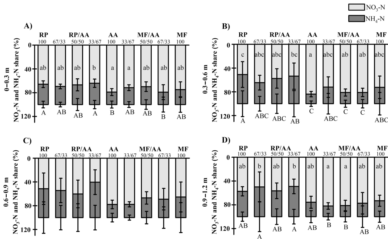
FIGURE 7 \text{NO}_3\text{-N} to \text{NH}_4\text{-N} (%) share in total \text{N}_{\min} at different soil depths in the 2021 field trial on September 14, 2021: (A) 0–0.3 m, p_{\text{NO}_3\text{-N}} = 0.04 , p_{\text{NH}_4\text{-N}} = 0.04 ; (B) 0.3–0.6 m, p_{\text{NO}_3\text{-N}} = 0.003 , p_{\text{NH}_4\text{-N}} = 0.003 ; (C) 0.6–0.9 m, p_{\text{NO}_3\text{-N}} = 0.09 , p_{\text{NH}_4\text{-N}} = 0.09 ; and (D) 0.9–1.2 m, p_{\text{NO}_3\text{-N}} = 0.001 , p_{\text{NH}_4\text{-N}} = 0.001 . One-factor analysis with Tukey's honestly significant difference (HSD). Means \pm standard deviation. Lowercase letters a and b indicate significance of \text{NO}_3\text{-N} (%) within the same sub-figure. Uppercase letters A and B indicate significance of \text{NH}_4\text{-N} (%) within the same sub-figure. Numbers 67/33, 50/50, and 33/67 indicate mixture proportions in percent, and 100 indicates a pure stand. AA, alfalfa pure stand; MF, meadow fescue; MF/AA, meadow fescue/alfalfa mixtures; RP, ribwort plantain pure stand; RP/AA, ribwort plantain/alfalfa mixtures.
