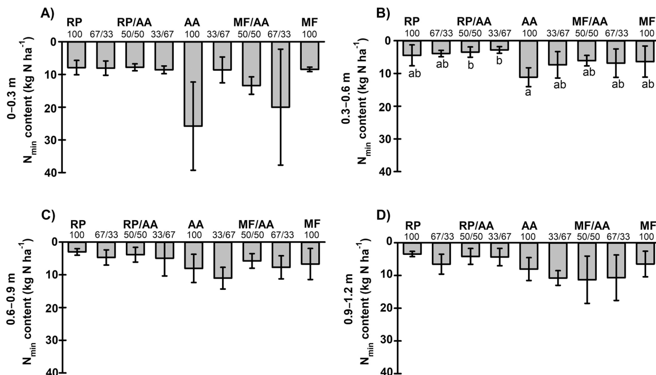
FIGURE 4 Plant-available mineral nitrogen ( N_{\min} ) content ( \text{kg N ha}^{-1} ) at different soil depths in the 2021 field trial on September 14, 2021: (A) 0–0.3 m, p = 0.11 ; (B) 0.3–0.6 m, p = 0.03 ; (C) 0.6–0.9 m, p = 0.07 ; and (D) 0.9–1.2 m, p = 0.4 . One-factor analysis with Tukey's honestly significant difference (HSD). Means \pm standard deviation. Lowercase letters a and b indicate significance within the same sub-figure. Numbers 67/33, 50/50, and 33/67 indicate mixture proportions in percent, and 100 indicates a pure stand. AA, alfalfa pure stand; MF, meadow fescue; MF/AA, meadow fescue/alfalfa mixtures; RP, ribwort plantain pure stand; RP/AA, ribwort plantain/alfalfa mixtures.
