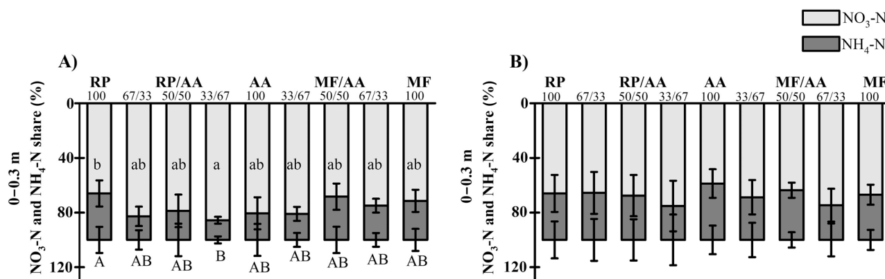
FIGURE 5 \text{NO}_3\text{-N} to \text{NH}_4\text{-N} (%) share in total N_{\min} at a 0- to 0.3-m soil depth in field trials in 2019 and 2021: (A) 0–0.3 m on June 27, 2019, p_{\text{NO}_3\text{-N}} = 0.02 , p_{\text{NH}_4\text{-N}} = 0.02 ; and (B) 0–0.3 m on May 25, 2021, p_{\text{NO}_3\text{-N}} = 0.76 , p_{\text{NH}_4\text{-N}} = 0.76 . One-factor analysis with Tukey's honestly significant difference (HSD). Means \pm standard deviation. Lowercase letters a and b indicate the significance of \text{NO}_3\text{-N} (%) within the same sub-figure. Uppercase letters A and B indicate the significance of \text{NH}_4\text{-N} (%) within the same sub-figure. Numbers 67/33, 50/50, and 33/67 indicate mixture proportions in percent, and 100 indicates a pure stand. AA, alfalfa pure stand; MF, meadow fescue; MF/AA, meadow fescue/alfalfa mixtures; RP, ribwort plantain pure stand; RP/AA, ribwort plantain/alfalfa mixtures.
