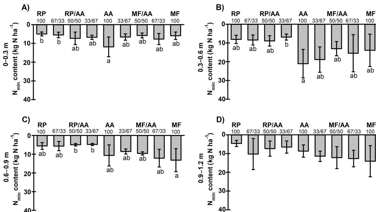
FIGURE 3 Plant-available mineral nitrogen ( N_{min} ) content ( \text{kg N ha}^{-1} ) at different soil depths in the 2019 field trial on October 16, 2019: (A) 0–0.3 m, p = 0.03 ; (B) 0.3–0.6 m, p = 0.01 ; (C) 0.6–0.9 m, p = 0.01 ; (D) 0.9–1.2 m, p = 0.16 . One-factor analysis with Tukey's honestly significant difference (HSD). Means \pm standard deviation. Lowercase letters a and b indicate significance within the same sub-figure. Numbers 67/33, 50/50, and 33/67 indicate mixture proportions in percent, and 100 indicates a pure stand. AA, alfalfa pure stand; MF, meadow fescue; MF/AA, meadow fescue/alfalfa mixtures; RP, ribwort plantain pure stand; RP/AA, ribwort plantain/alfalfa mixtures.
