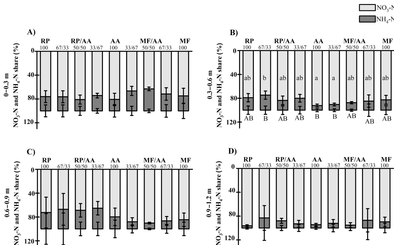
FIGURE 6 \text{NO}_3\text{-N} to \text{NH}_4\text{-N} (%) share in total \text{N}_{\min} at different soil depths in the 2019 field trial on October 16, 2019: (A) 0–0.3 m, p_{\text{NO}_3\text{-N}} = 0.14 , p_{\text{NH}_4\text{-N}} = 0.14 ; (B) 0.3–0.6 m, p_{\text{NO}_3\text{-N}} = 0.01 , p_{\text{NH}_4\text{-N}} = 0.01 ; (C) 0.6–0.9 m, p_{\text{NO}_3\text{-N}} = 0.1 , p_{\text{NH}_4\text{-N}} = 0.1 ; (D) 0.9–1.2 m, p_{\text{NO}_3\text{-N}} = 0.16 , p_{\text{NH}_4\text{-N}} = 0.16 . One-factor analysis with Tukey's honestly significant difference (HSD). Means \pm standard deviation. Lowercase letters a and b indicate the significance of \text{NO}_3\text{-N} (%) within the same sub-figure. Uppercase letters A and B indicate the significance of \text{NH}_4\text{-N} (%) within the same sub-figure. Numbers 67/33, 50/50, and 33/67 indicate mixture proportions in percent, and 100 indicates a pure stand. AA, alfalfa pure stand; MF, meadow fescue; MF/AA, meadow fescue/alfalfa mixtures; RP, ribwort plantain pure stand; RP/AA, ribwort plantain/alfalfa mixtures.
