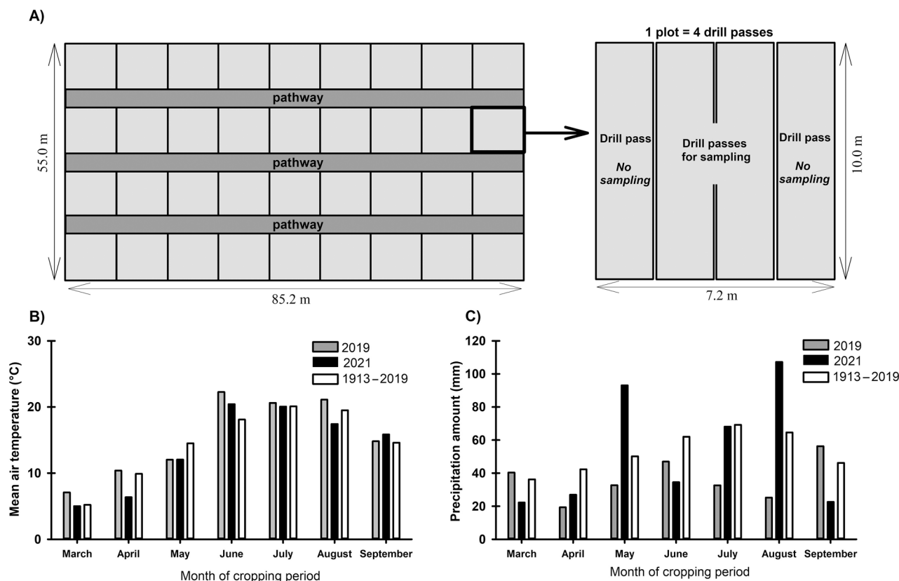
FIGURE 1 (A) Experimental design as a randomized block (85.2 m × 55 m) with each plot (7.2 m × 10 m) consisting of four drill passes. (B) Mean monthly temperature and long-term temperature mean (°C) and (C) mean monthly precipitation and long-term mean of precipitation amount (mm) graphs for field trials at Canitz, Germany, from March to September 2019 and 2021. Weather data source: Wassergut Canitz GmbH.
