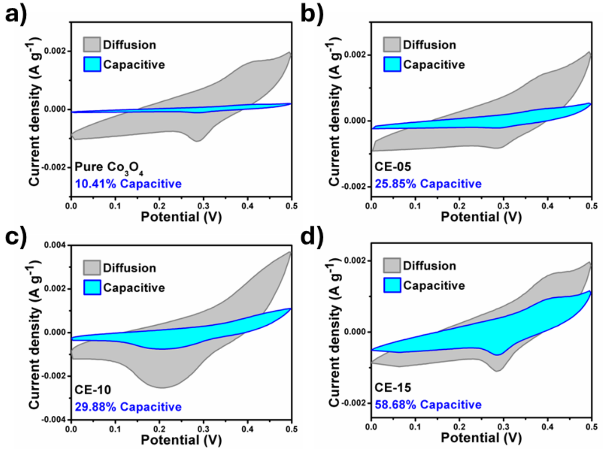
Figure (S5). (a-d) The diffusion and capacitive plots of pure Co 3 O 4 nanostructures and different (CE-05, CE-10, and CE-15, CE stands for cobalt oxide rotten solanum melongenas juice) at various scan rates in 3M KOH solution .
