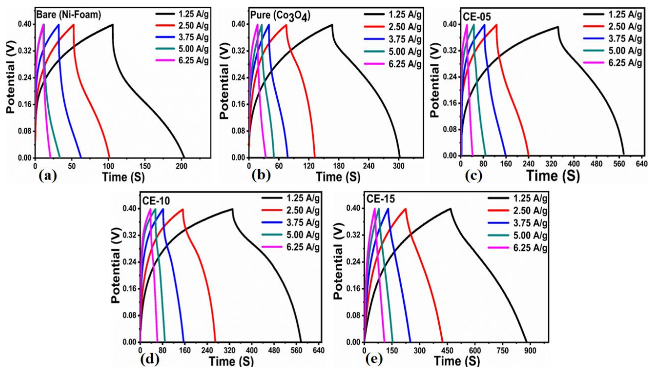
Figure. 7: (a-e) \text{Co}_3\text{O}_4 nanostructures with different volumes and without rotten solanum melongena juice like (CE-05, CE-10, CE-15, CE-20, CE stands for cobalt oxide-solanum melongena juice for the illustration of redox aspects using GCD curves at various current densities in 3.0 M KOH aqueous solution.
