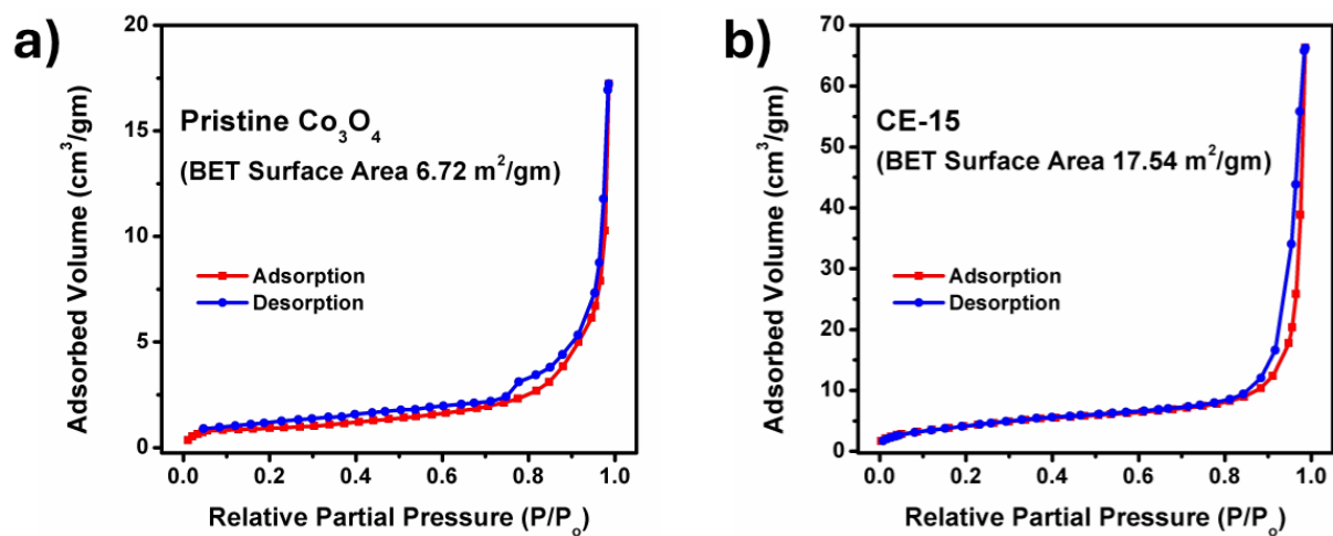
Figure 5: BET surface area analysis of pure \text{Co}_3\text{O}_4 nanostructures and 15 mL rotten solanum melongena juice mediated \text{Co}_3\text{O}_4 nanostructures.
