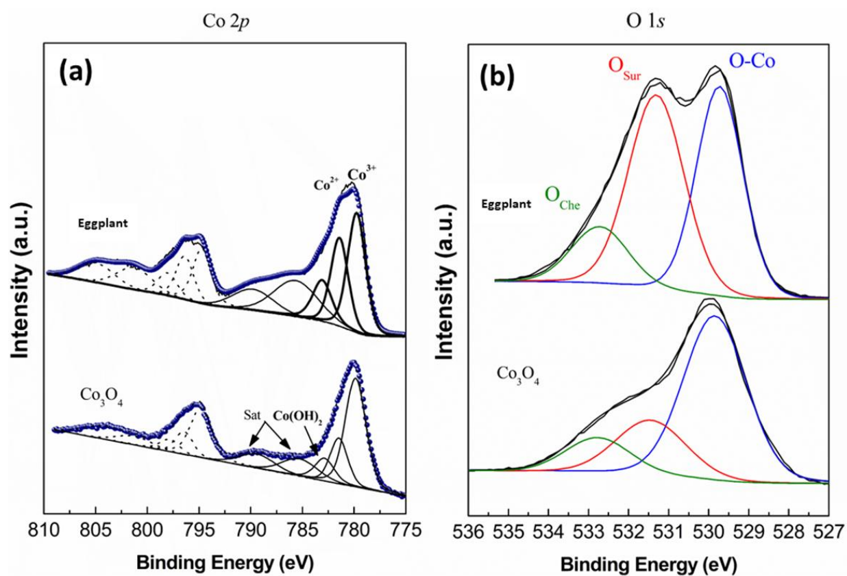
Figure 4: X-ray core level spectra of pure \text{Co}_3\text{O}_4 nanostructures and 15 mL rotten solanum melongena juice mediated \text{Co}_3\text{O}_4 nanostructures (a) Co 2p_{3/2} , (b) O 1s.
