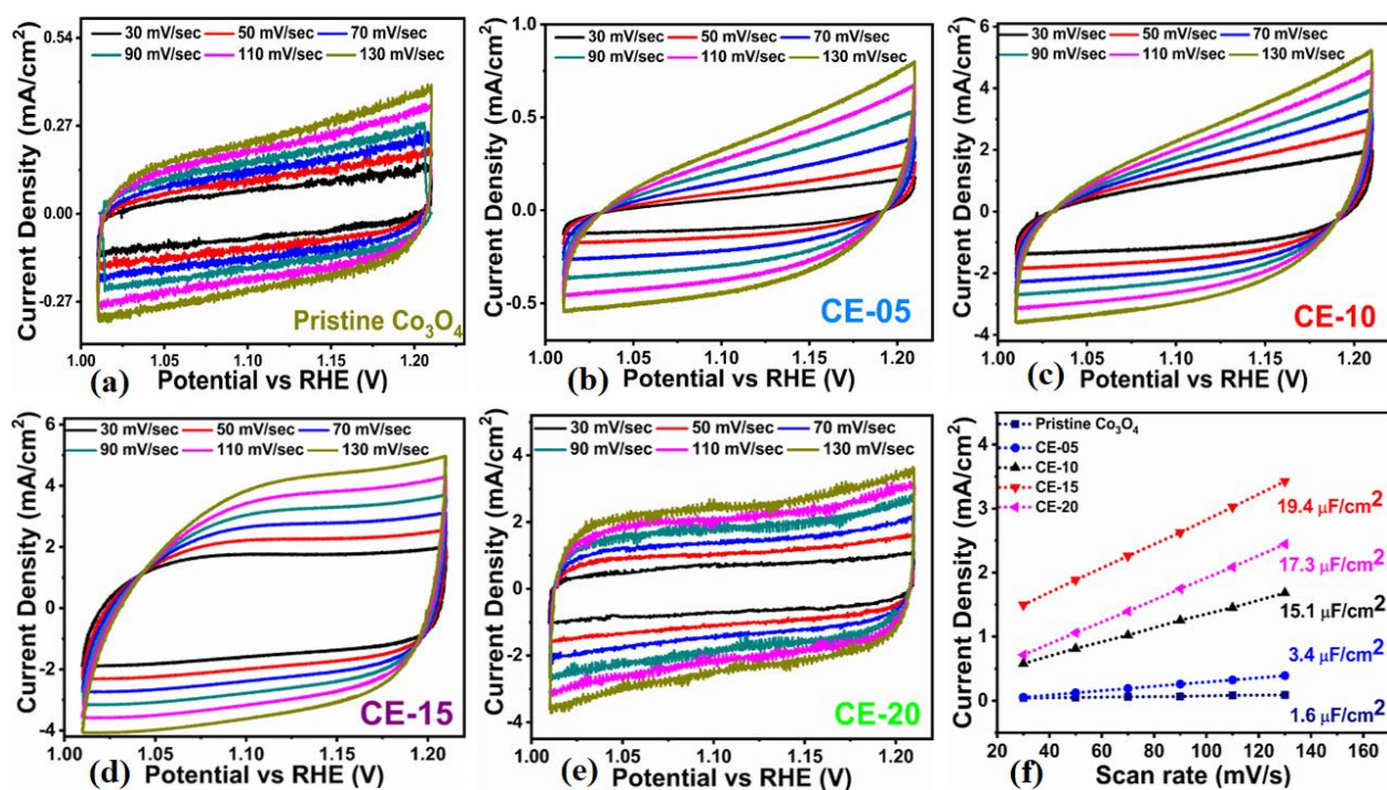
Figure (S2). (a-e) CV curves of \text{Co}_3\text{O}_4 nanostructures with different volumes and without rotten solanum melongenas juice like (CE-05, CE-10, CE-15, CE-20, CE stands for cobalt oxide) at various scan rates, (f) Related linear plot for the calculation of ECSA from the non-Faradic region of CV curves of \text{Co}_3\text{O}_4 nanostructures with different volumes and without rotten solanum melongenas juice.
