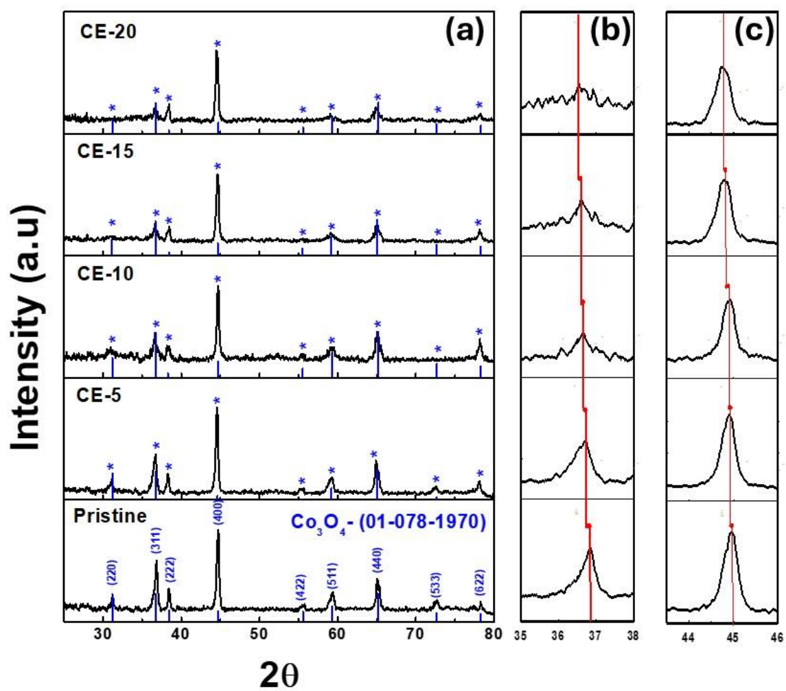
Figure 1: (a) XRD patterns of Co 3 O 4 synthesized without rotten solanum melongena juice (pristine) and with 5 mL (CE-5), 10 mL (CE-10), 15 mL (CE-15) and 20 mL (CE-20) of rotten solanum melongenas juice. (b) (311) plane peak shift of corresponding XRD patterns, (c) (400) plane main peak shift of corresponding XRD patterns.
