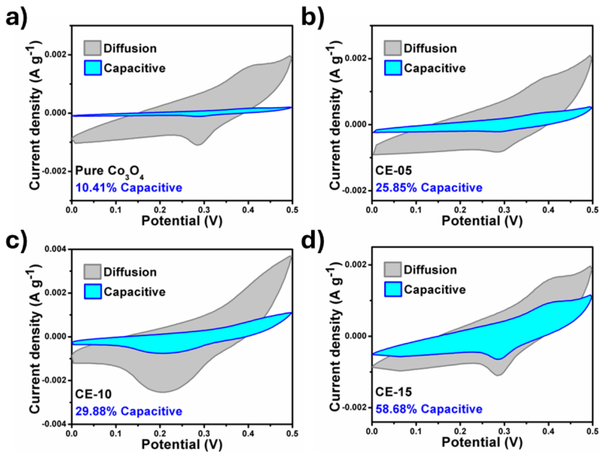
Figure (S4): (a-d) The illustration of diffusion and capacitive distribution of pure \text{Co}_3\text{O}_4 nanostructures and different (CE-05, CE-10, and CE-15) at 60 mV/s in 3M KOH solution.
