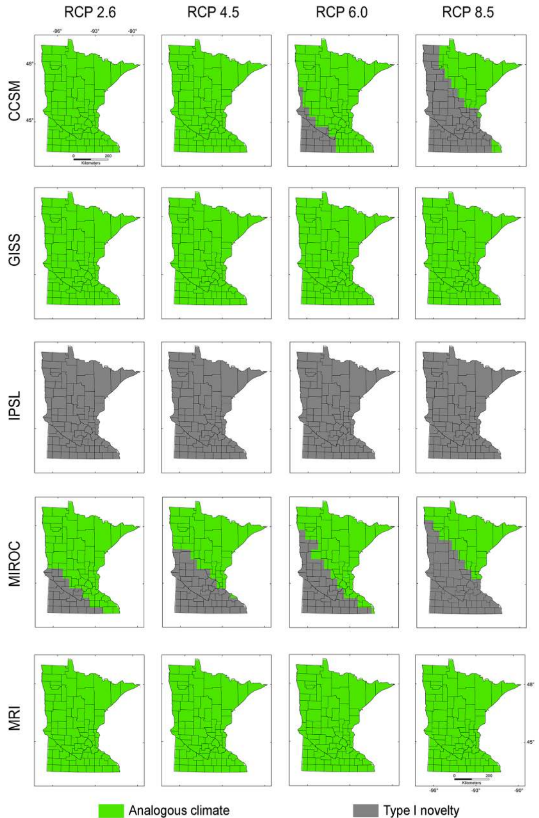
Fig 4. Environmental similarity comparison between the calibration M 7 and the projection region of Minnesota. Exdet tool identified analogous climates between present-day climate in the calibration region from the
