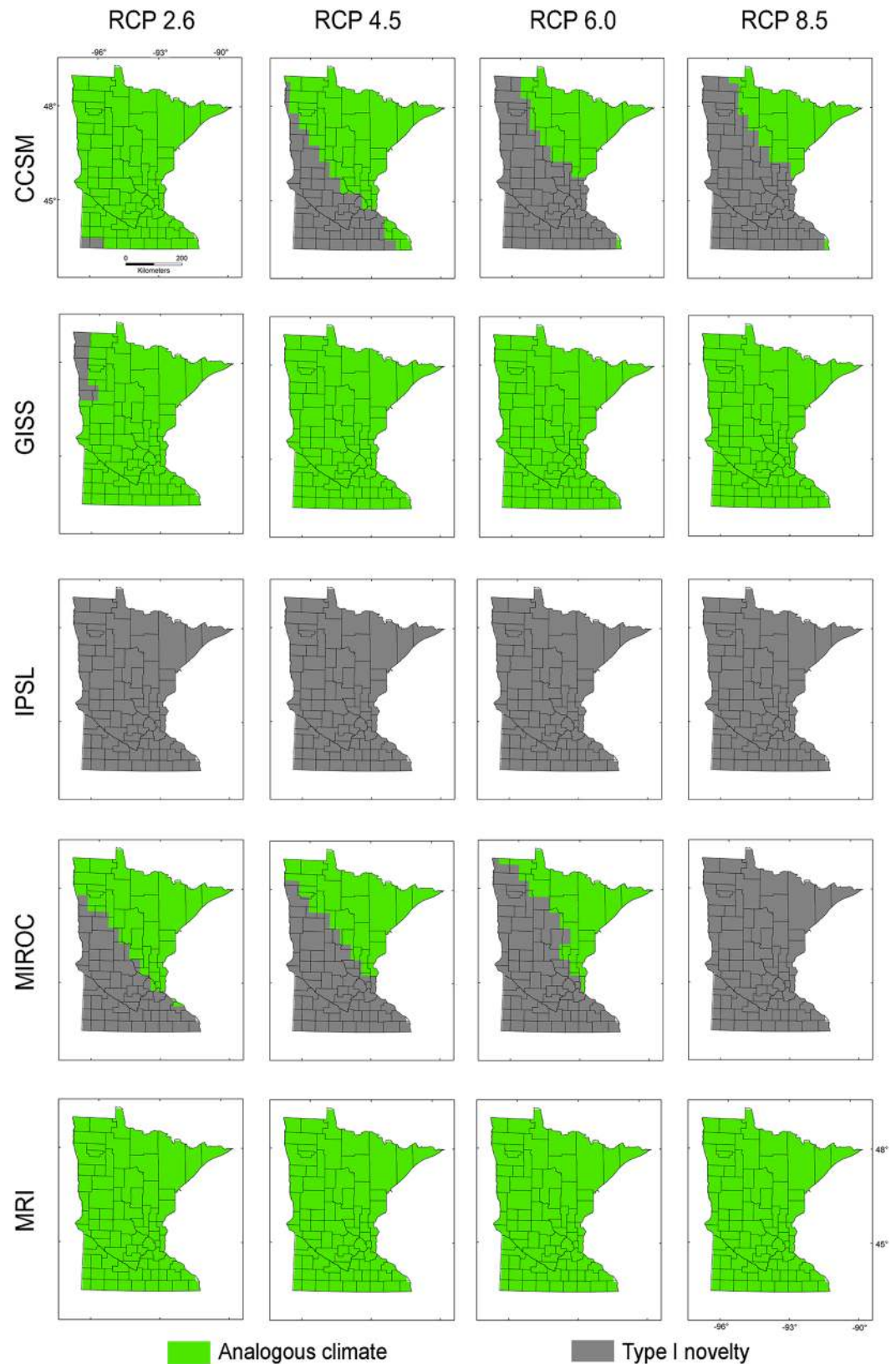
Fig 6. Environmental similarity comparison between the calibration M_0 and the projection region of Minnesota. Legend as in Fig 3.
