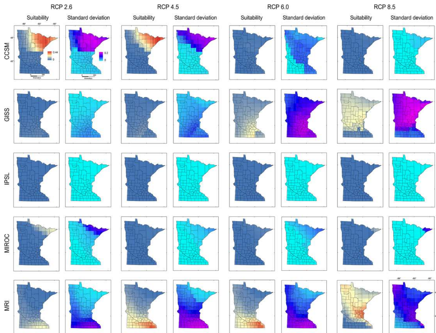
Fig 7. Ecological niche models of starry stonewort calibrated in M_1 and projected to future climate scenarios in Minnesota. Ecological niche model predictions based on model calibration region M_1 projected to Minnesota. Areas with high (red) or low (blue) environmental suitability (Suitability, left) and high (pink) or low (light blue) model uncertainty (Standard deviation, right) were identified for five future climate models (i.e., CCSM, GISS, IPSL, MIROC, MRI) and four RCP scenarios of CO 2 emissions (i.e., 2.6, 4.5, 6, and 8.5).
