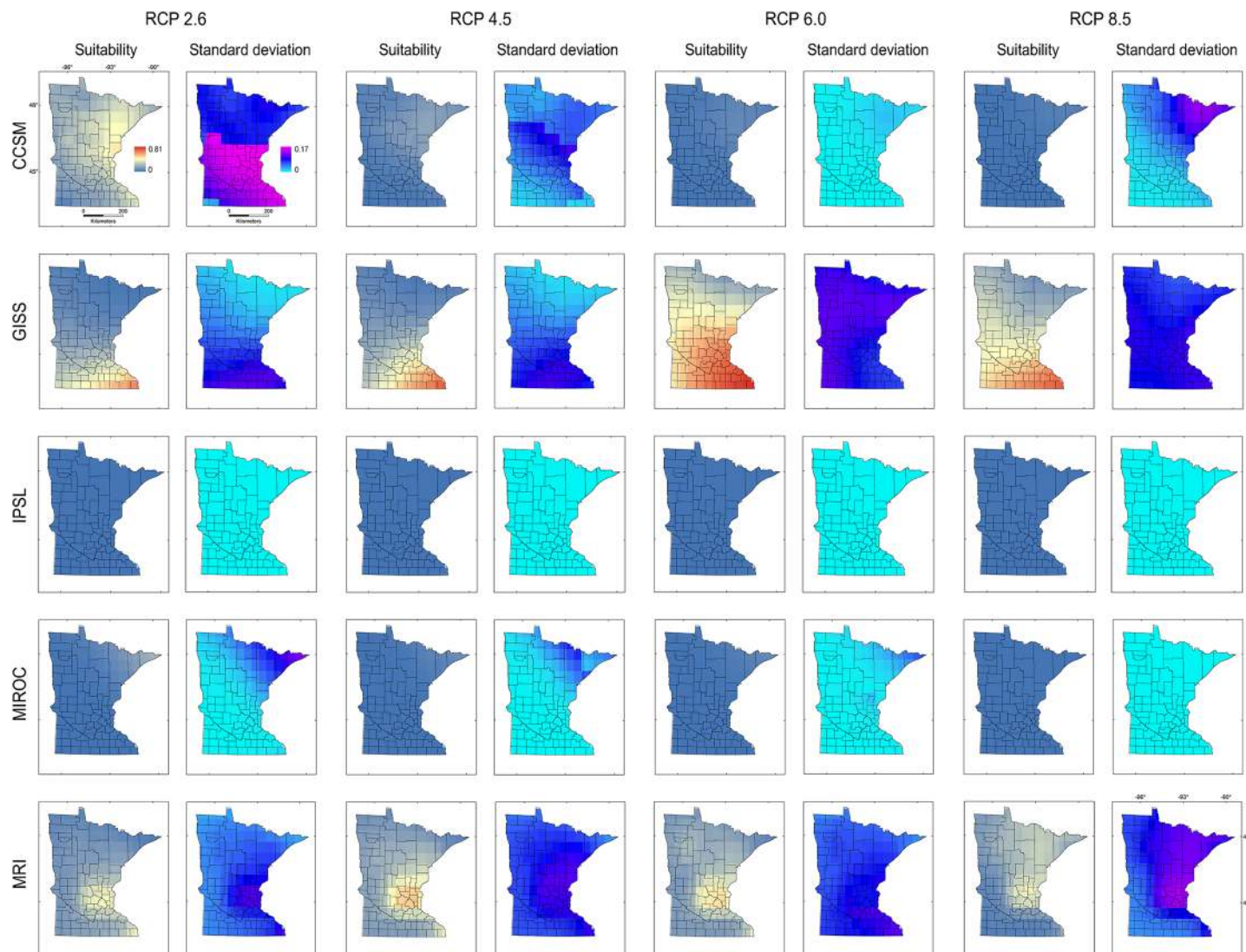
Fig 9. Ecological niche models of starry stonewort calibrated in M_g and projected to future climate scenarios in Minnesota. Ecological niche model predictions based on model calibration region M_g projected to Minnesota. Legend as in Fig 7.
