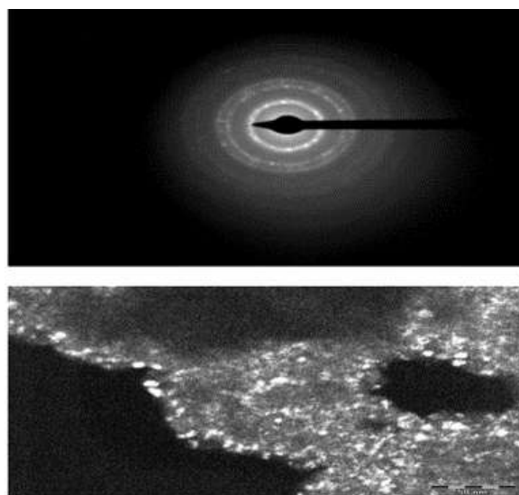
Fig 5: TEM image of Murraya Koenigii capped CdS nanoparticles.[18]
