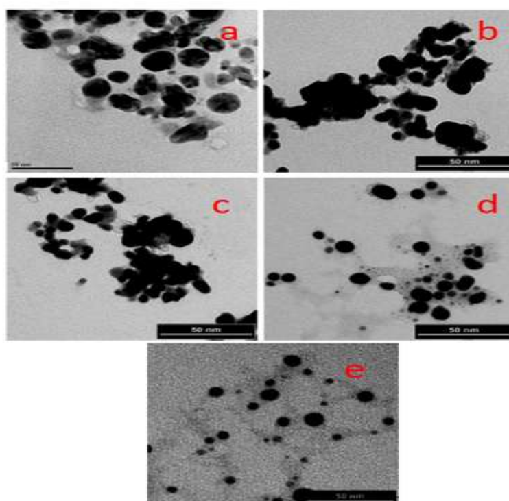
Fig 8: TEM images of the biosynthesized silver nanoparticles.[21]
