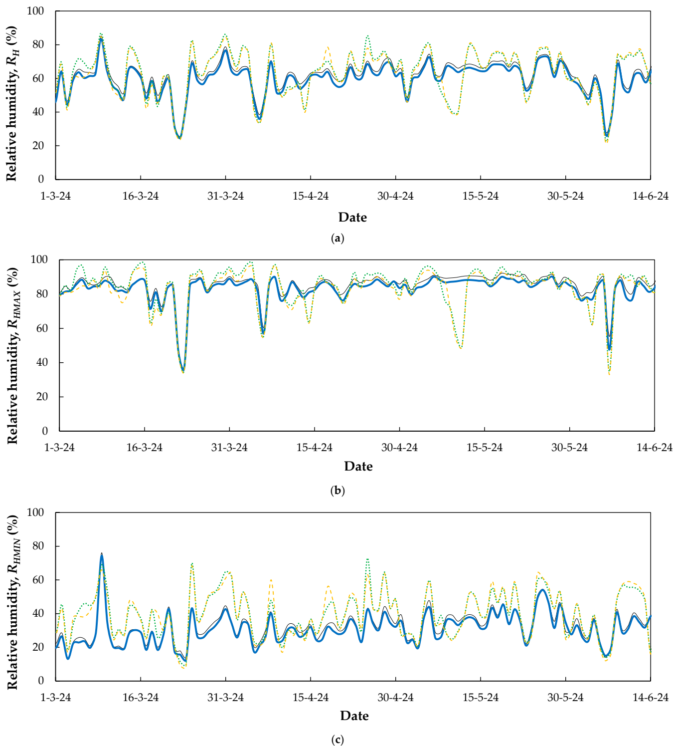
Figure 5. Evolution of daily mean (a), maximum (b), and minimum (c) relative humidity values recorded at 9 m height (---) and 5 m height (....), and inside the greenhouse: eastern sector with black polypropylene mulch (—) and western sector with white polyethylene mulch (—).
