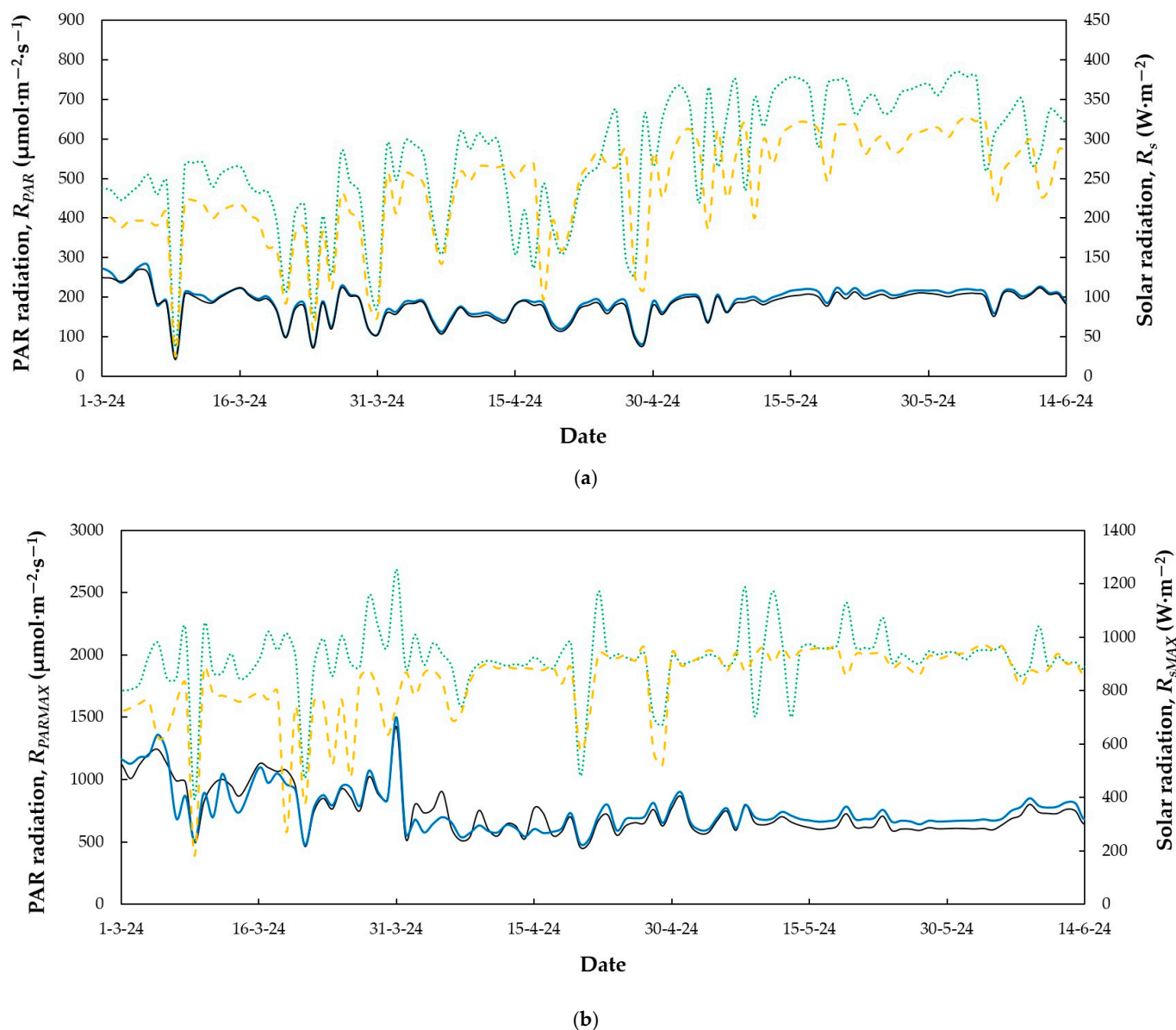
Figure 3. Evolution of mean (a) and maximum (b) PAR values recorded outdoors at 5 m height (····) and inside the greenhouse: eastern sector with black polypropylene mulch (—) and western sector with white polyethylene mulch (—). External solar radiation measured at 9 m height (---).
