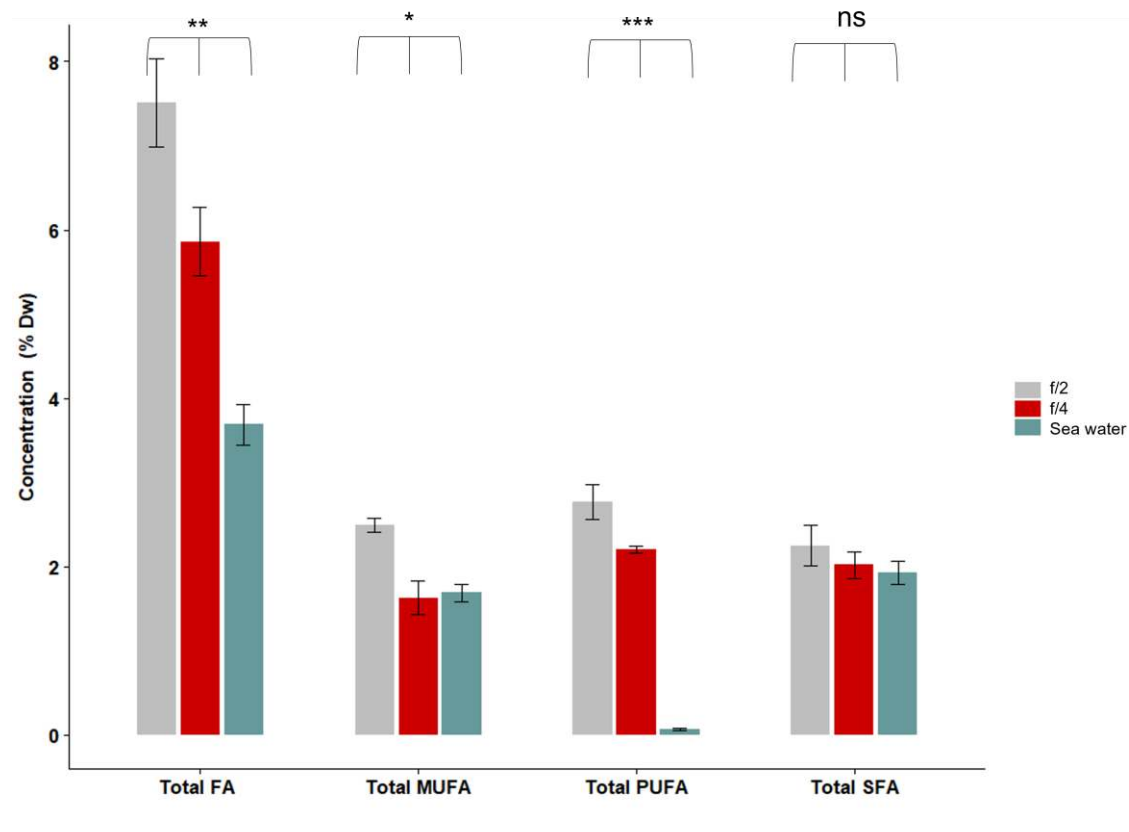
Figure 6.5. Total fatty acid content (FA), monounsaturated fatty acid (MUFA), polyunsaturated fatty acid (PUFA) and the saturated fatty acid (SFA) of Symsagittifera roscoffensis cultured in different media (f/2, f/4, or plain seawater). Total fatty acid content, monounsaturated fatty acid, polyunsaturated fatty acid was significantly different when S. roscoffensis was grown in different media. Saturated fatty acid was not significantly different when S. roscoffensis was grown in different media. Asterisks indicate significant differences (ANOVA: * p < 0.05 ; ** p < 0.01 ; *** p < 0.001 ; ns not significant). N=200 worms per experiment. Data are presented as % dry weight (DW; mean \pm s.e.).
