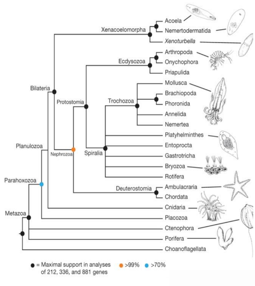
Figure 1.2. The phylogenetic position of Xenacoelomorpha within Bilateria (From Cannon et al. , 2016).
