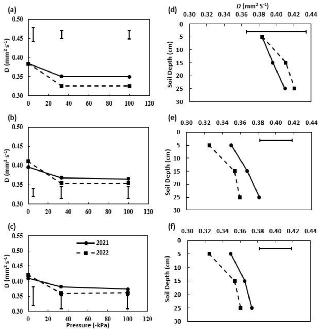
Fig. 4. Soil thermal diffusivity ( D ) for cover crops during 2021 and 2022 at (a) 0-10 cm, (b) 10-20, and (c) 20-30 cm depths, and at (d) 0 kPa, (e) -33 kPa, and (f) -100 kPa soil water pressures. Least square difference (at p < 0.05 ) among the study years is indicated by bars.
