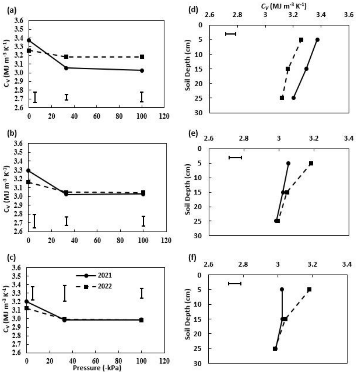
Fig. 3. Volumetric heat capacity ( C_v ) for cover crops during 2021 and 2022 at (a) 0-10 cm, (b) 10-20, and (c) 20-30 cm depths, and at (d) 0 kPa, (e) -33 kPa, and (f) -100 kPa soil water pressures. Least square difference (at p < 0.05 ) among the study years is indicated by bars.
