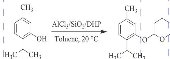
Scheme 8. Tetrahydropiranylation of thymol aided by \text{AlCl}_3/\text{SiO}_2 .
