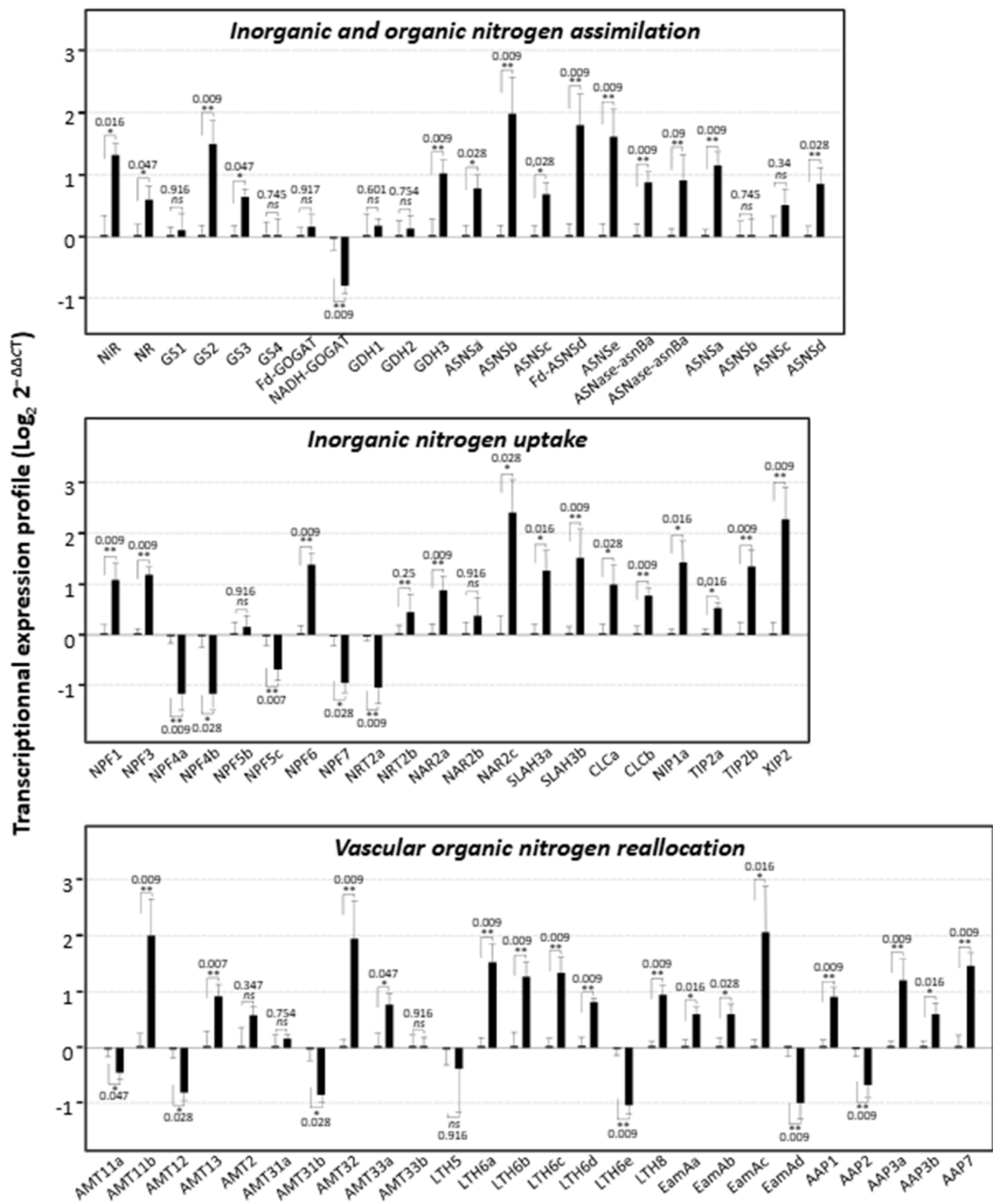
Fig. 4 Quantitative real-time RT-PCR of selected genes related to nitrogen transport, assimilation, and vascular release. Transcript abundances of the genes were recorded by real-time q RT-PCR analyses, relative to those of the control, using the 2^{-\Delta\Delta CT} method. The significant differences were statistically analyzed between untreated and treated roots with Molinia exudate. Each biological condition comprised five biological replicates, with each replicate representing a pooled sample of six randomly selected seedlings (Kruskal & Wallis, adjusted p -value < 0.05)
