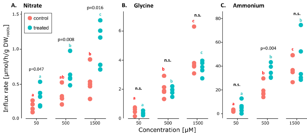
Fig. 2 Influx rates of nitrate (A), glycine (B), and ammonium (C) in excised fine roots of oak seedlings in response to different concentrations of nitrogen sources. p -values indicate significance of differences between treatments at the same concentration (n.s. = p -value above 0.05). Lowercase letters indicate significance levels between concentrations for the same treatment modality
