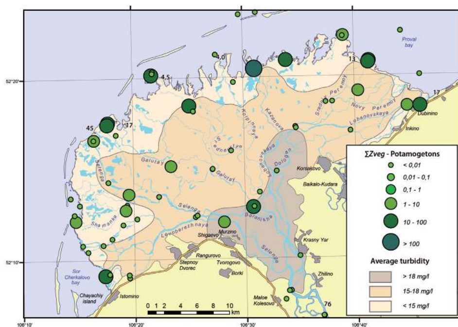
Fig. 7. Spatial distribution of the additive coefficient Z_{veg} in hydatophytes by the example of pondweeds
