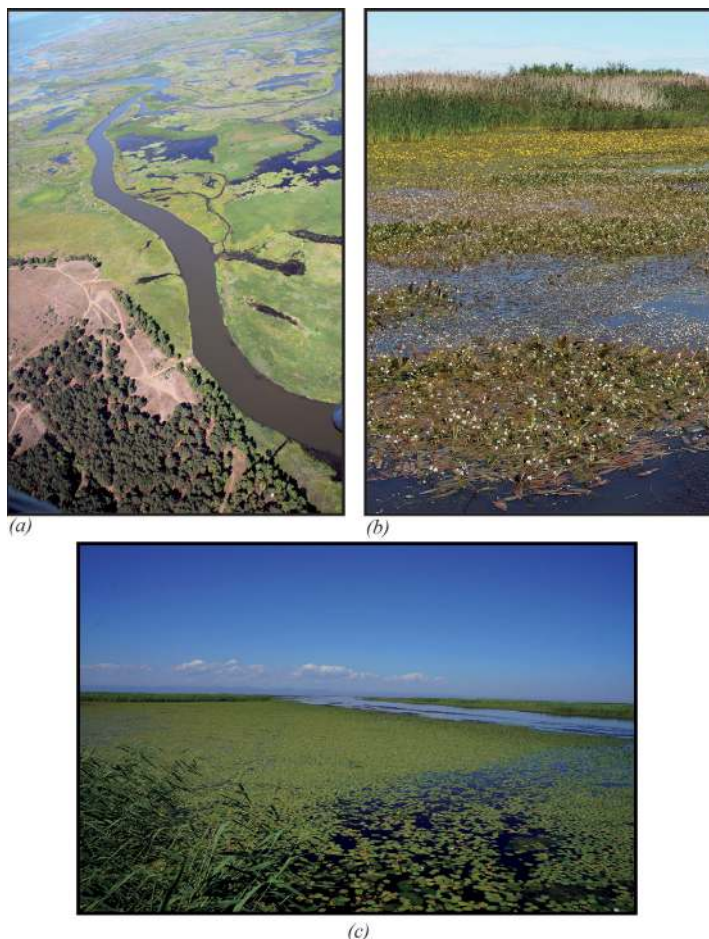
Fig. 2. Aquatic vegetation of the Selenga delta:
