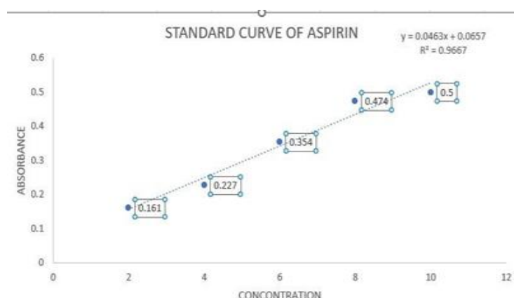
Standard Curve of Aspirin
