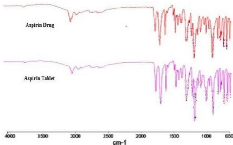
FTIR of aspirin and aspirin tablet
