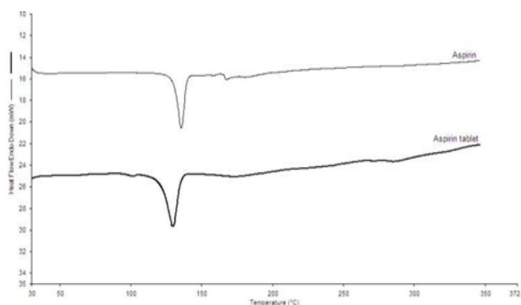
DSC of Aspirin and Aspirin Tablet.
