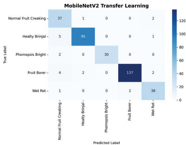
Figure 9. Confusion matrices for MobileNetV2 under transfer learning on test set.
