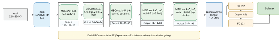
Figure 6. Schematic of the EfficientNetB0 architecture with MBConv blocks.
