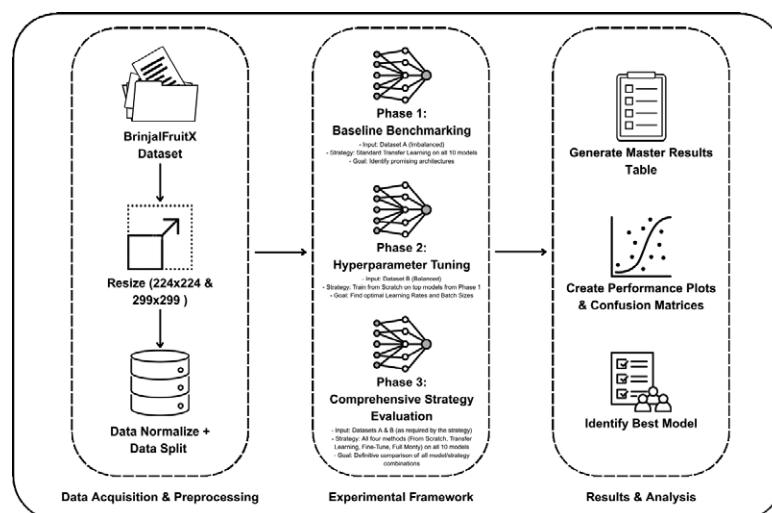
Figure 1. Workflow for brinjal fruit disease classification.
