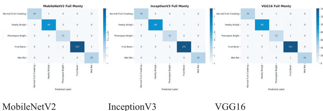
Figure 10. Confusion matrices for top-performing models under the Full Monty strategy on the test set.
