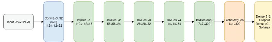
Figure 7. Schematic of the MobileNetV2 architecture with depth wise separable convolutions and inverted residuals.
