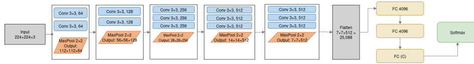
Figure 3. VGG16 architecture with stacked 3 \times 3 convolutional layers.
