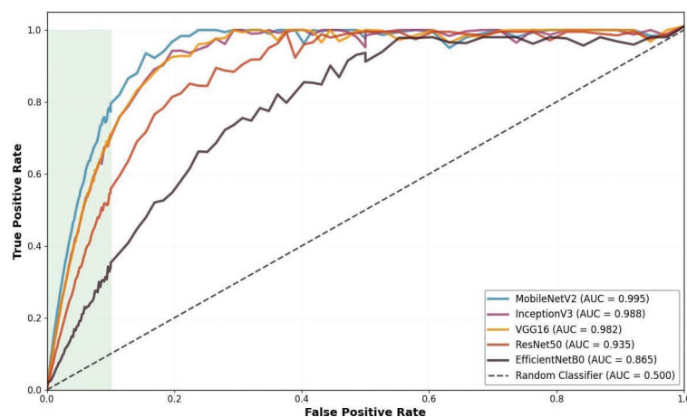
Figure 11. ROC curves for representative models under their best strategies.
