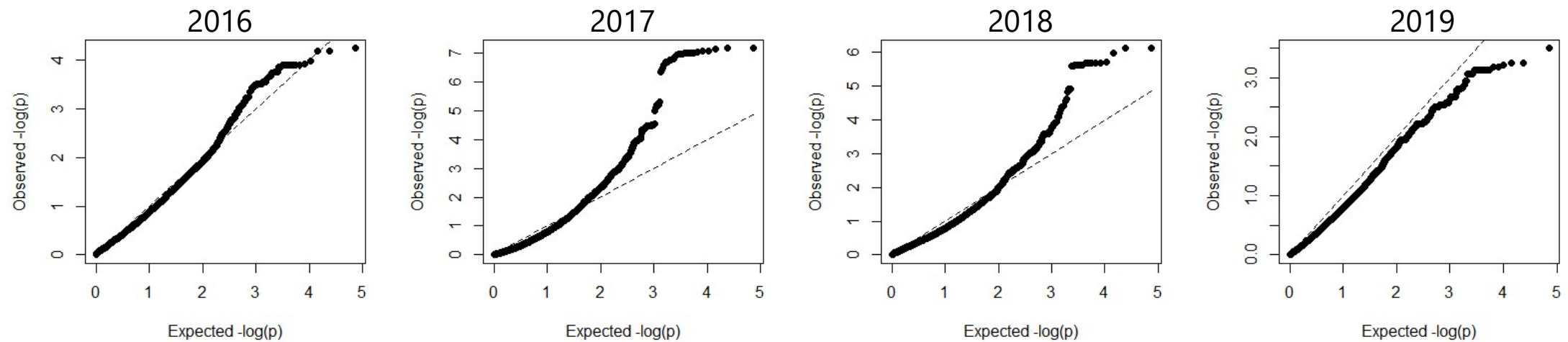
Figure S2. Quantile-Quantile (Q-Q) plots for genome-wide association analyses of scab resistance traits.
