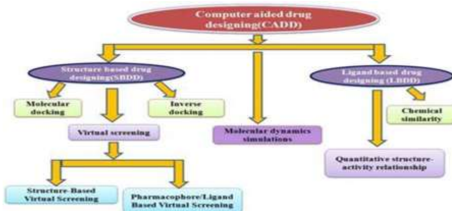
Figure no.2 Computer Aided Drug Desing
