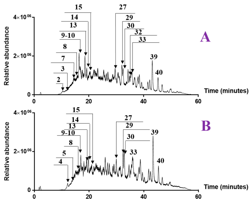
Figure 3. LC-MS chromatograms of ethyl acetate extracts of A. henoniana stems; (A) stems collected in winter (February 2021); (B) stems collected in spring (May 2021).
