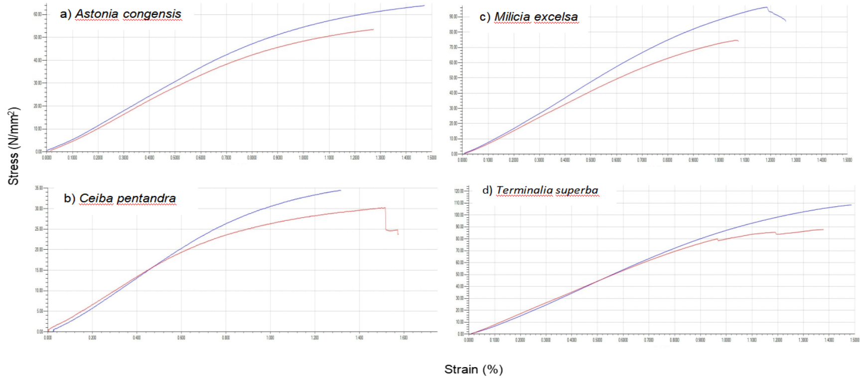
Figure 1: the 3-point flexural test of wood materials sourced from four indigenous timber species.
