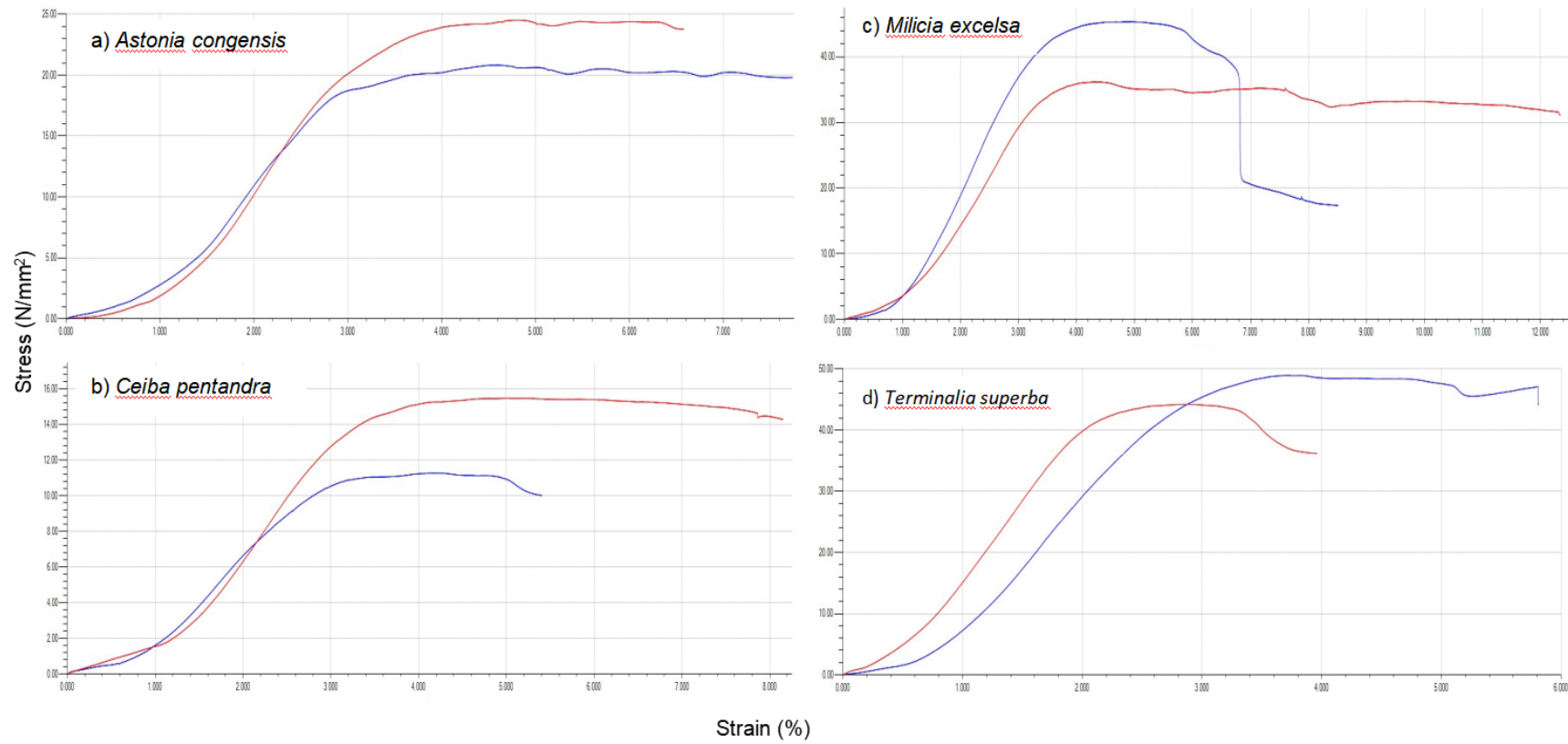
Figure 2: Axial Compression test for wood materials sourced from four indigenous timber species.
