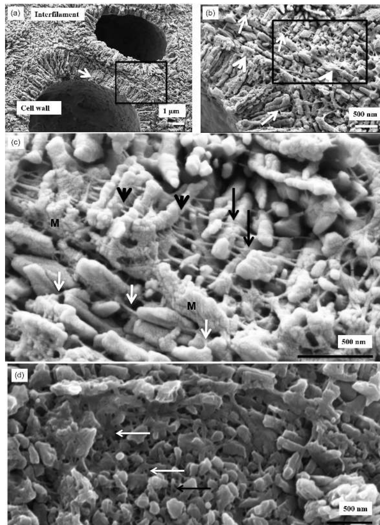
Figure 7. K. epilaeve cell wall structure. Crust polished and cleaned for 2 min. (a) Cell walls have radial Mg-calcite, whereas the interfilament grains are orientated either parallel to the filament axis or randomly within the corner junctions. Within the radial cell walls a secondary concentric banding pattern is visible (white arrow). Black box enlarged in (b). (b) Organic fibrils, ~10 nm wide, run parallel to cell wall edges (black arrows). Fibrils are concentrated along the outer of the cell wall (white arrows). Black box enlarged in (c). (c) The cell wall fibrils appear to string through the centre of the radial grains (black arrowheads); other fibrils drape over the grains (black arrows). Fibrils are present in the interfilament (white arrows). M – mineralised membrane. (d) Plan view of cell wall grains. Organic fibrils form a dense mesh (white arrows).
