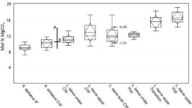
Figure 6. Box plot of EDS mol % MgCO 3 results. Boxes represent the second and third quartiles. The lower and upper bars are the minimum and maximum values (excluding an outlier for L. laeve under cell wall). The solid middle line within the box is the median value and the dash middle line the average. The dashed diamond box represents one standard deviation. The drawn-on cross represents the XRD mol % (X) and the seasonal range (a) of mol % for the Arctic Bay–Kingitok–Quirpon dataset in Fig. 5.
