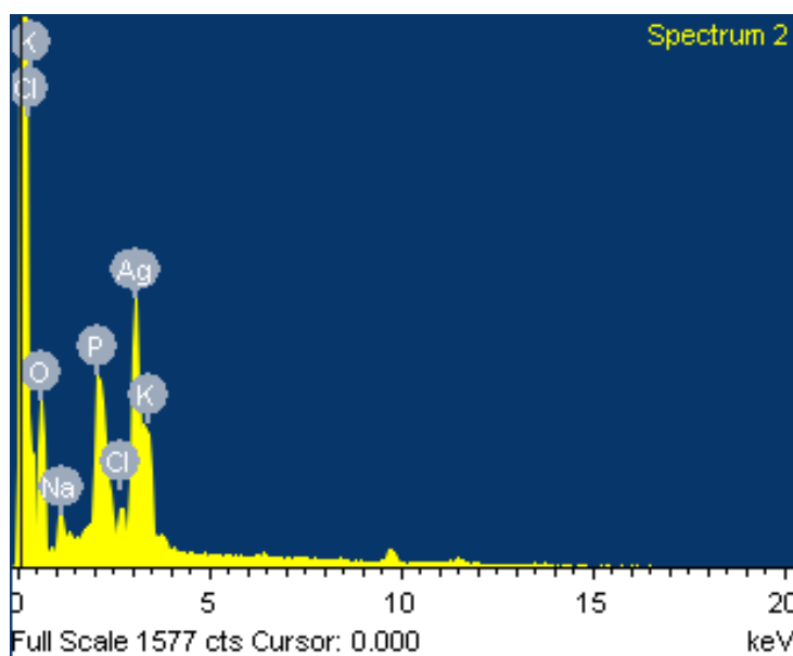
Figure 3. EDX- spectra of Ipomoea pes-tigris synthesized silver nanoparticles was showed reducing \text{Ag}^+ to \text{Ag}^0 .
