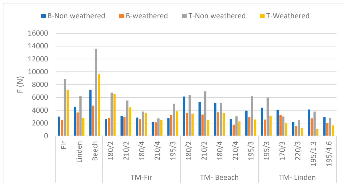
Figure 2. Comparison of the bending and tensile force results of the weathered and non-weathered specimens under laboratory conditions.
