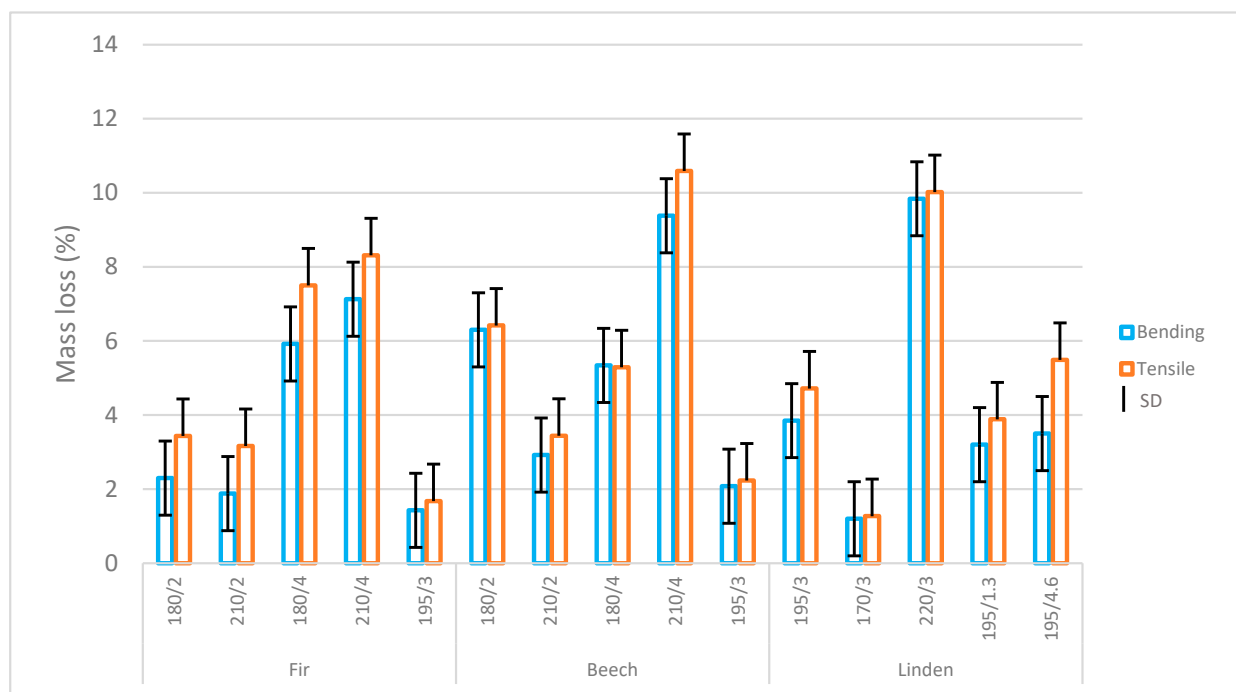
Figure 1. Mass loss of fir, linden, and beech wood after thermal modification.
