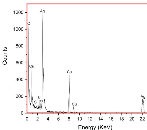
Figure 4. EDX spectrum of AgNPs synthesized by Carya Illinoensis Extract.
