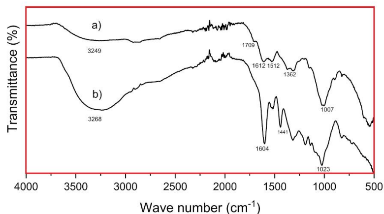
Figure 5. FT-IR of (a) silver nanoparticles and (b) Carya Illinoensis Extract.
