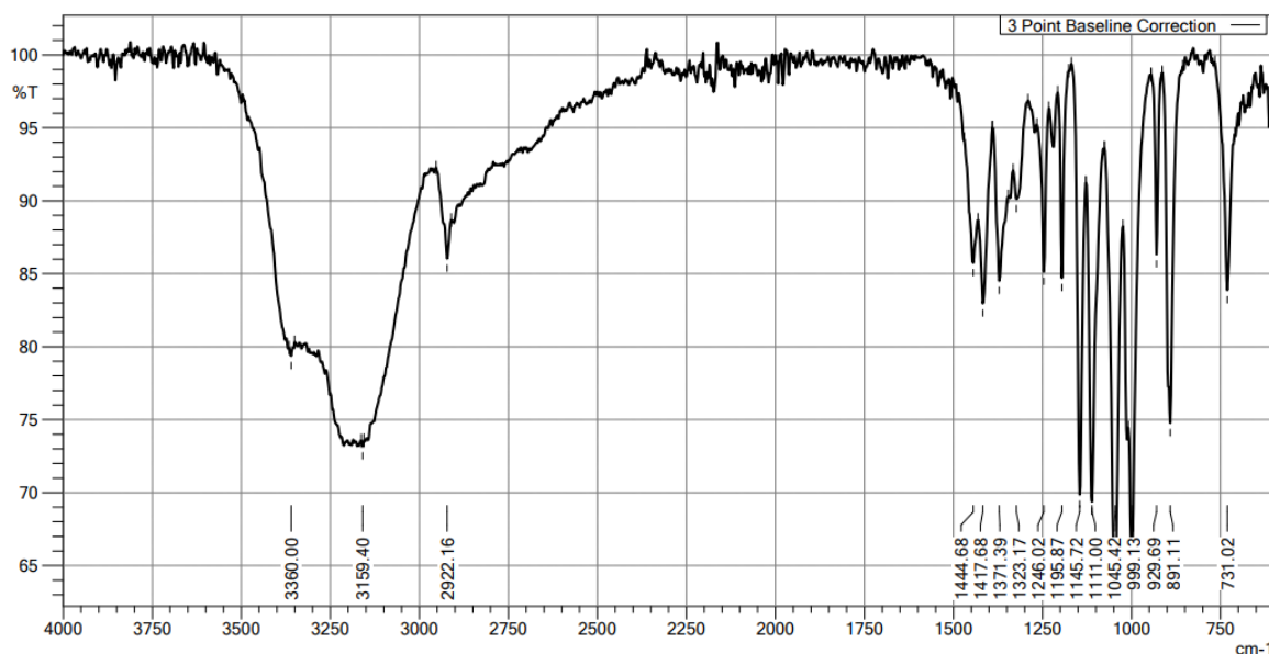
Figure 3: IR spectrum of compound (1).
